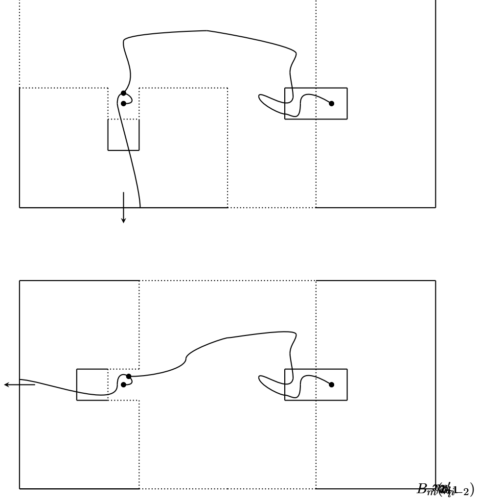
Figure 1: Configuration within B_m(x_{i-1}) \cup B_m(x_i) on the event G_0 \cap \dots \cap G_i .
