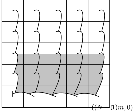
Figure 2: The tree \mathcal{U}_{N,m} on the event F(N, m) .
