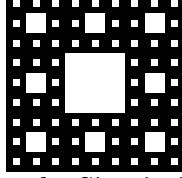
Figure 2: The Sierpinski carpet
