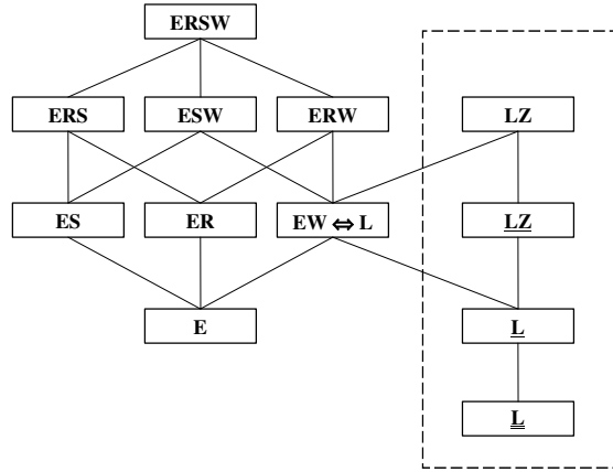
Fig. 1 Tree of nonlocally-related systems of nonlinear elasticity.
