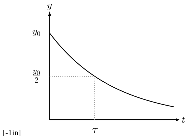
Figure 11.2: Half-life in an exponentially decreasing process.
