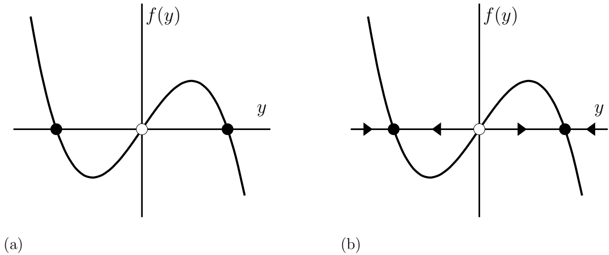
Figure 13.2: Where y is increasing, decreasing, or static
