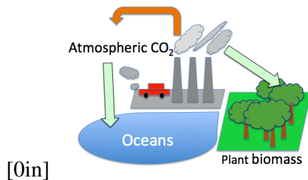
Figure 11.14: \text{CO}_2 is produced by emissions from burning fossil fuel and other human activities (orange arrow). The oceans and plant biomass are both sinks that absorb \text{CO}_2 (light green arrows).
