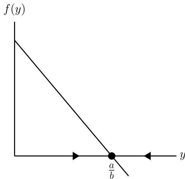
Figure 13.4: Qualitative sketch for a DE
