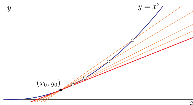
Secants approaching a tangent line
