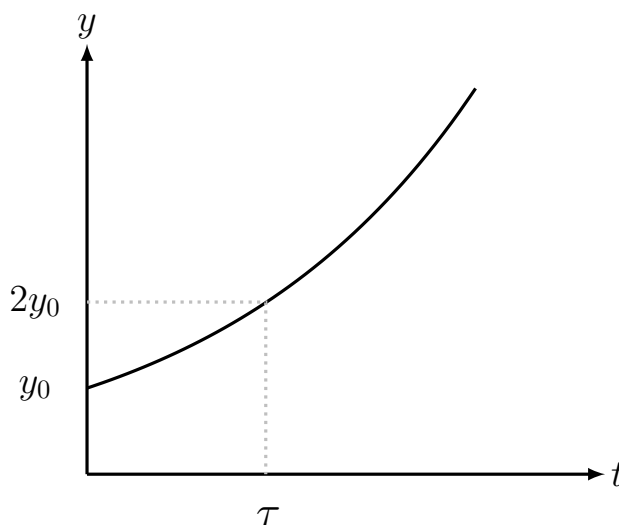
Figure 11.13: Doubling time for exponential growth.
