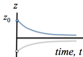
Figure 11.5: The deviation away from steady state (blue, grey curves) is z(t) = y(t) - a/b . We can solve the differential equation for z(t) because it is a simple exponential decay equation. Here we show two typical solutions for z .
