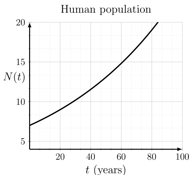
Figure 11.12: Projected world population
