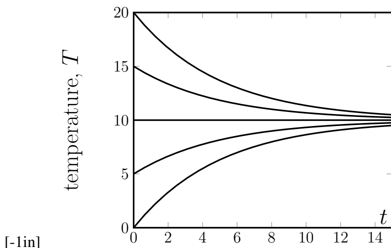
Figure 11.8: Temperature versus time, T(t) , for a cooling object.
