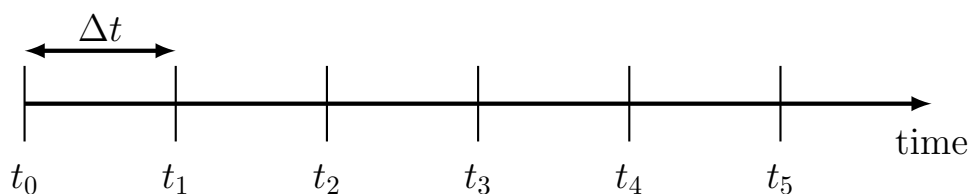
Figure 12.1: The time axis is subdivided into steps of size \Delta t .
