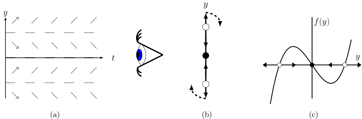
Figure 13.1: Slope field related to state space
