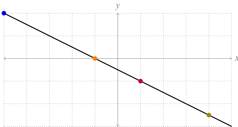
Figure 3.1: Line with points
