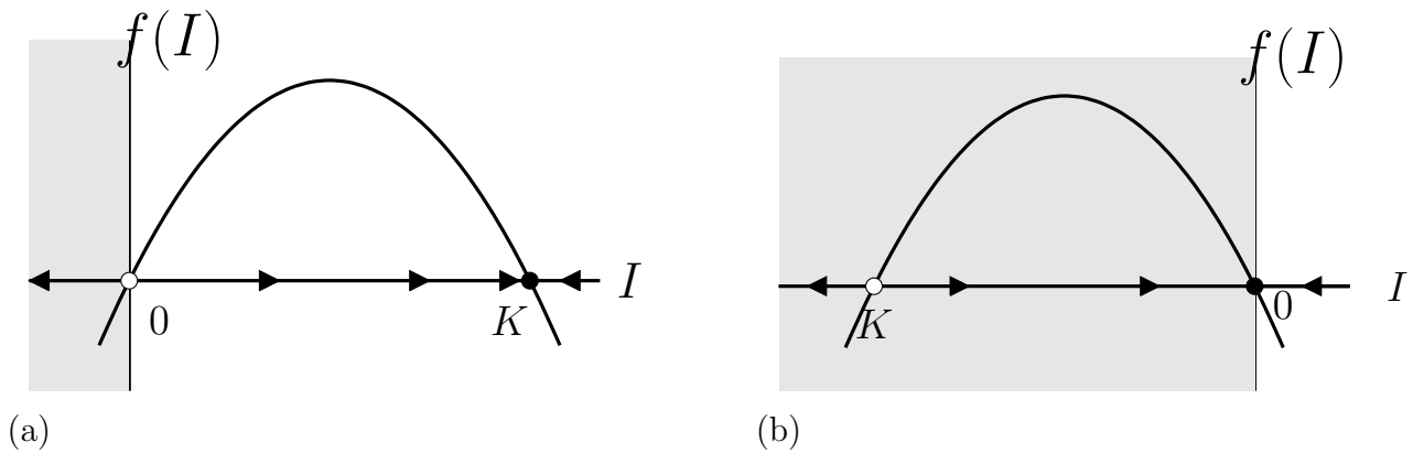
Figure 13.7: State-space diagrams for differential equation (13.3.2). Plots of f(I) as a function of I in the cases (a) K \geq 0 , and (b) K < 0 . The grey regions are not biologically meaningful since I cannot be negative.
