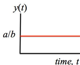
Figure 11.3: y = a/b is a constant solution to the differential equation in (11.4.1). We call this type of solution a steady state .
