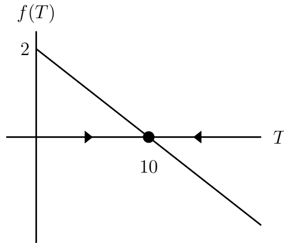
Figure 13.3: Determining flow direction
