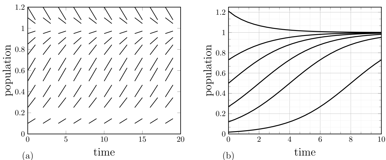
Figure 13.6: (a) Slope field and (b) solution curves for the logistic equation (13.2.1), \frac{dy}{dt} = 0.5 \cdot y(1 - y)
