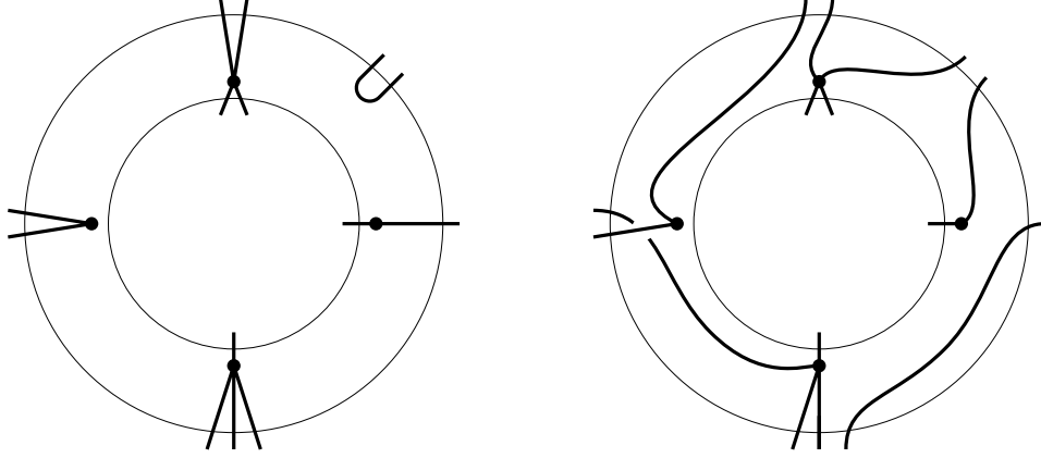
two annular graphs of type 10, (4,2,4,2) , (2,1,3,2)
