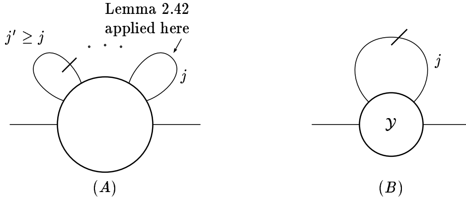
Figure 20: The case \tilde{G}(\phi) non-overlapping and D_h acting at root scale
