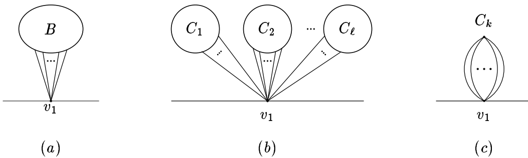
Figure 10: The case of one external vertex
