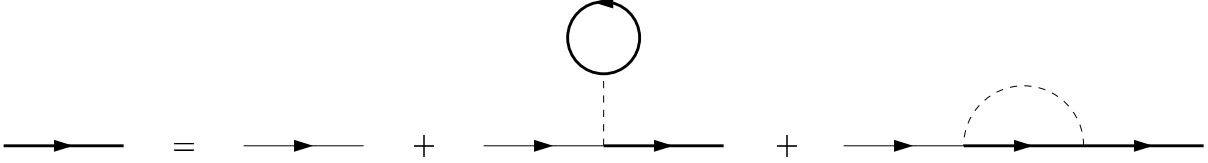
Figure 4: The Hartree-Fock equations
