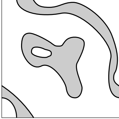
Figure 1: An example of a Fermi surface obeying A3
