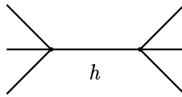
Figure 18: The six-legged scale h subgraph of Figure 16
