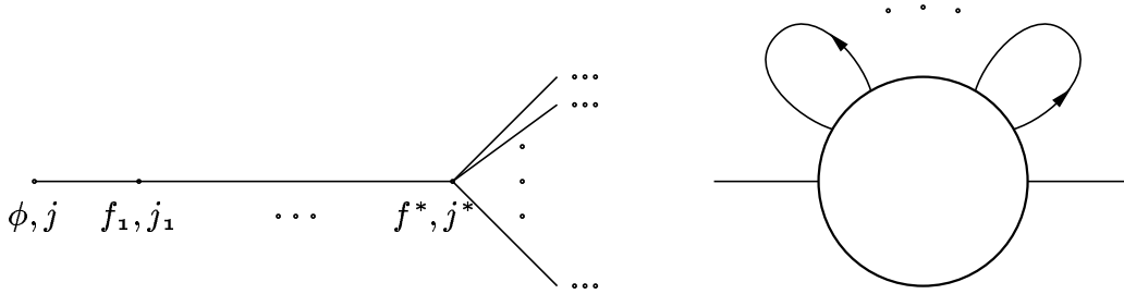
Figure 19: The case \tilde{G}(\phi) non-overlapping, P = 0
