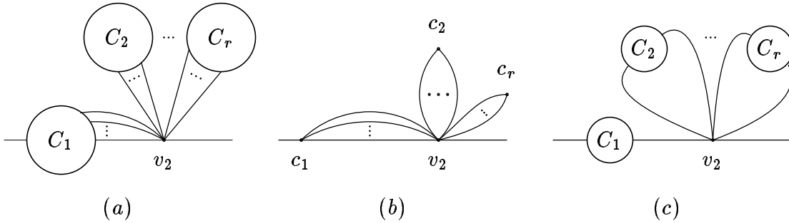
Figure 11: The case of two external vertices
