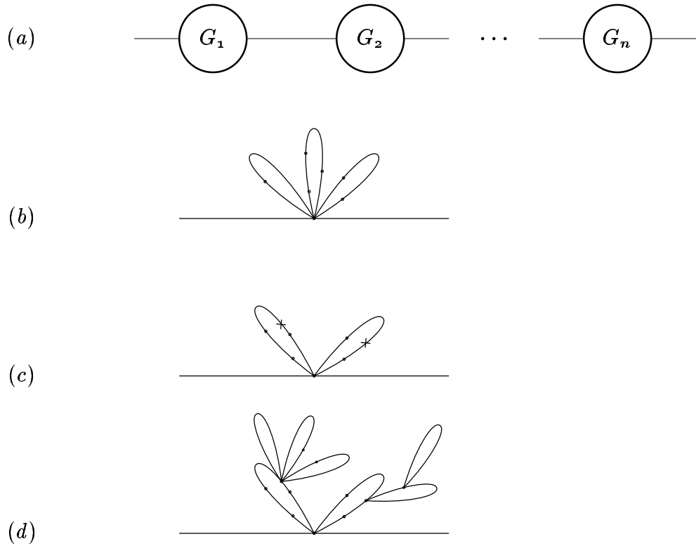
Figure 8 (a) A string of two-legged diagrams (b) An ST diagram (c), (d) GST diagrams
