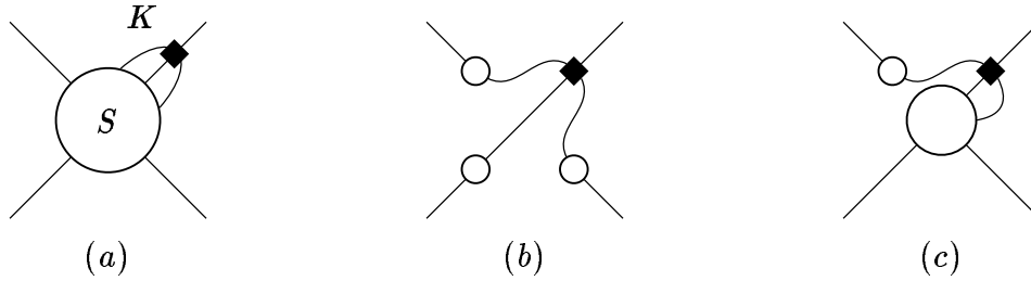
Figure 15: The case V_E(G') = 4
