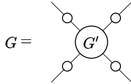
Figure 12: General form of a one-particle reducible four-legged graph
