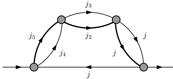
Figure 17: A particle–particle wicked ladder
