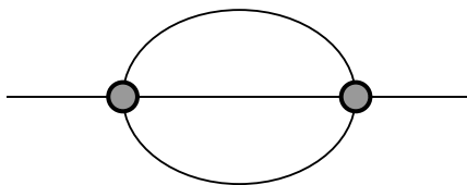
Figure 1: The sunset graph
