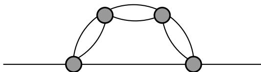
Figure 12: The wicked ladder. There may be an arbitrary number of bubbles
