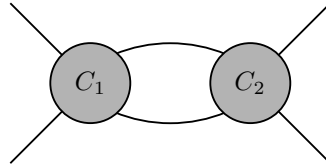
Figure 13: Two-particle reducible four-legged graphs
