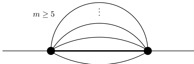
Figure 7: The multiple sunset
