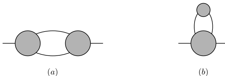
Figure 14: Two-particle reducible two-legged graphs
