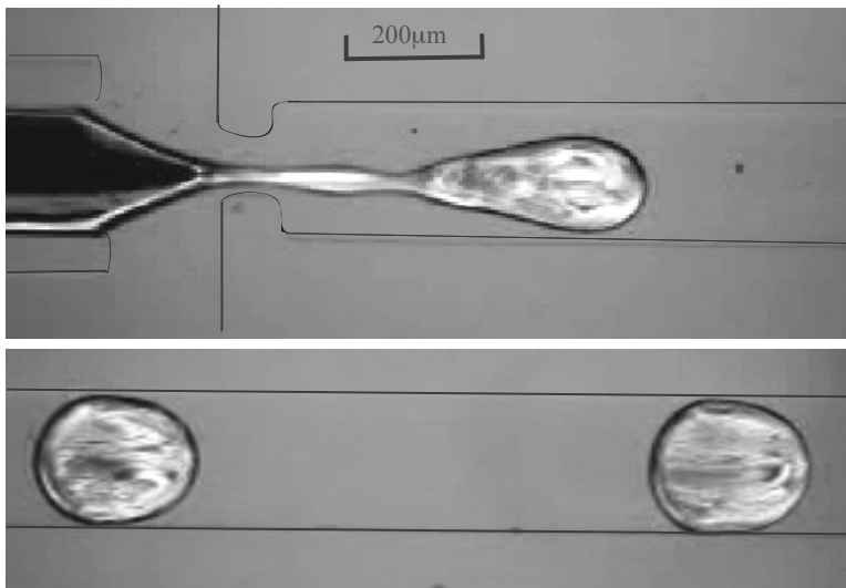
Figure 7: Liquid crystal droplet in the jetting regime pinching off after the orifice and traveling downstream. Bottom image shows droplets traveling downstream from the orifice. Flow rate of liquid crystal is 0.08 ml/hr, while flow rate of silicone oil is 0.25 ml/hr.
