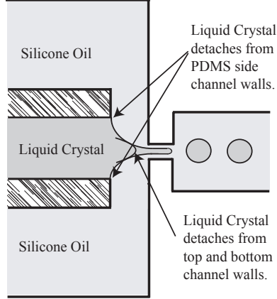
Figure 5: Schematic drawing of possible contact regions of liquid crystal phase with respect to PDMS walls that is related to surface hydrophobicity.
