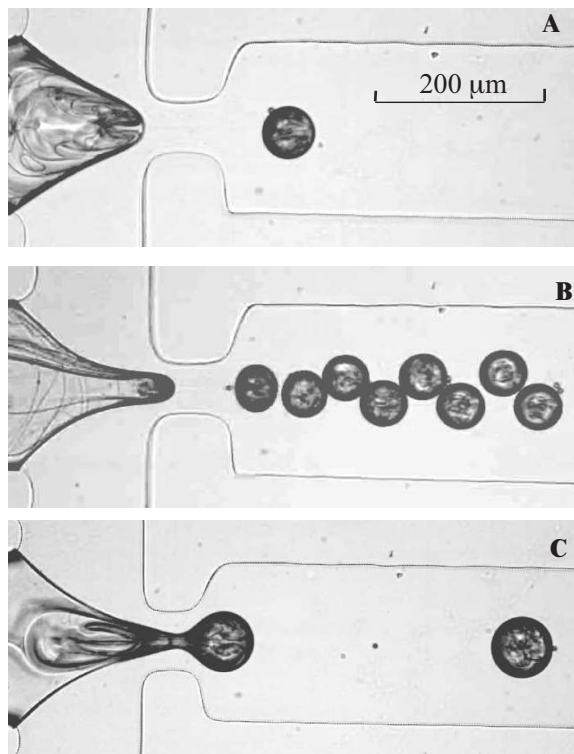
Figure 6: Nematic LC droplet formation in the dripping regime. A: nematic LC primary droplet pinching off at the orifice and traveling downstream. Flow rate of liquid crystal is 0.003 mL/hr, while flow rate of silicone oil is 0.04 mL/hr. B: nematic LC drops arrange themselves into two lines that move downstream of the orifice. Flow rate of liquid crystal is 0.01 mL/hr, while flow rate of silicone oil is 0.05 mL/hr. C: a single stream of nematic LC droplets forming at the orifice. Flow rate of liquid crystal is 0.001 mL/hr while the flow rate of the silicone oil is 0.05 mL/hr. The orifice size in these images is 60 \mu\text{m} . The scale bar applies to all three images.
