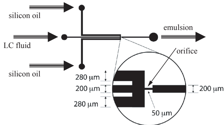
Figure 2: Microfluidic device used for droplet formation. The dispersed phase flows down the center channel and pinches off at the orifice, while the continuous phase flows down the two outside channels. The orifice size varies between 50\ \mu\text{m} to 60\ \mu\text{m} .
