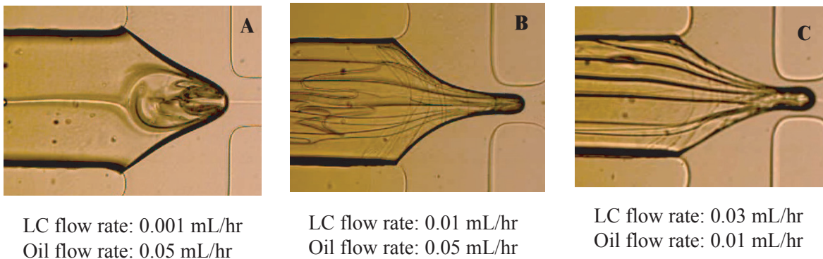
Figure 9: Images display the presence of defects with different defect strengths when the nematic liquid crystal filament is stretched into the orifice.
