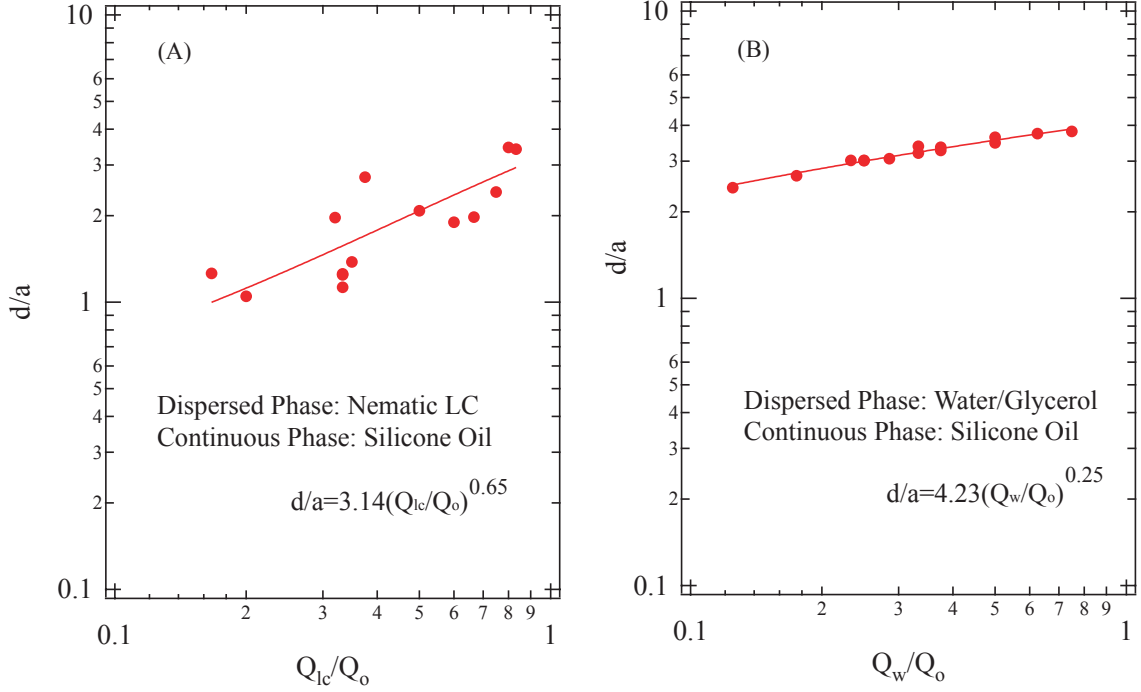
Figure 8: The ratio of the droplet diameter to the orifice width is plotted versus the ratio of the dispersed phase flow rate to the continuous phase flow rate. Figure A shows the results with liquid crystal as the dispersed phase and silicone oil as the continuous phase. The data covers both dripping and jetting regimes and the transition occurs roughly at \frac{Q_{Lc}}{Q_o} \approx 0.3 . Figure B shows the results with a water/glycerol solution as the dispersed phase and silicone oil as the continuous phase. Below both figures is the log-log plot of the data. The surface properties of the channel were hydrophobic.
