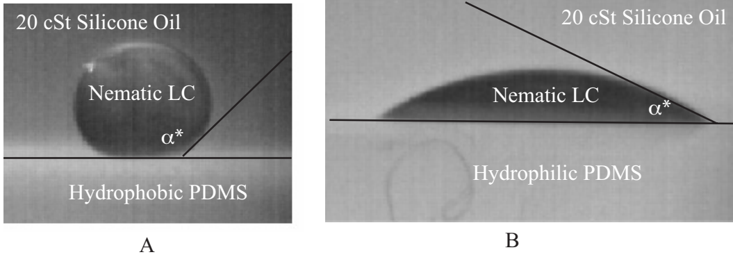
Figure 3: Images of liquid crystal droplets in contact with PDMS when immersed in silicone oil at room temperature. Image A shows the droplet in contact with hydrophobic PDMS, and image B shows the droplet in contact with hydrophilic PDMS.
