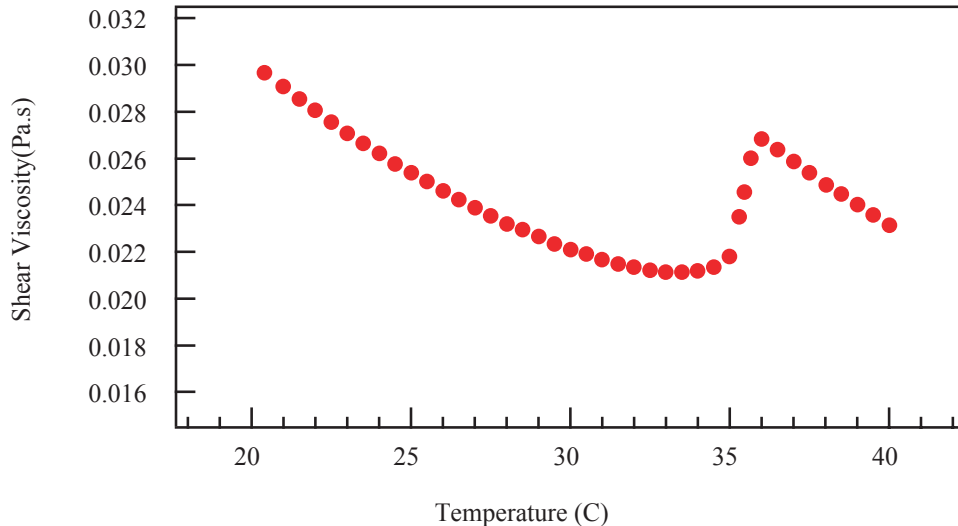
Figure 1: Rheology characterization of 5 CB under temperature sweep by using an AR2000 rheometer. The shear viscosity is the dissipative part of the complex viscosity in small-amplitude oscillation.
