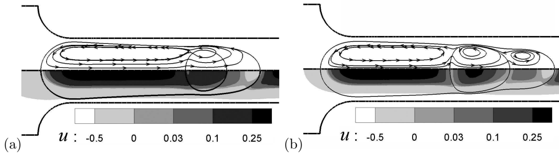
Figure 5: Flow fields inside the compound drop toward the end of the entry process for two core radii: (a) \zeta_c = 0.64 , (b) \zeta_c = 0.80 . In both cases, Ca = 0.179 , Re = 1.56 \times 10^{-2} . The streamlines are drawn in a reference frame fixed to the leading edge of the compound drop, which has an instant velocity of 0.81V in (a) and 1.21V in (b). The gray-scale contours are for the horizontal velocity u .
