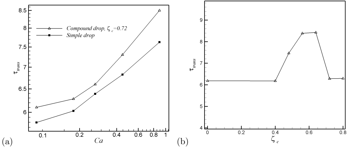
Figure 4: (a) Effect of the inner drop on the transit time with changing pressure drop with \zeta_c = 0.72 . The Reynolds number varies in the range 7.81 \times 10^{-3} \leq Re \leq 7.81 \times 10^{-2} . (b) Transit time as a function of the core radius, represented by \zeta_c , at Ca = 0.179 and Re = 1.56 \times 10^{-2} . In both plots the size of the outer drop is fixed with \zeta_s = 1.4 .
