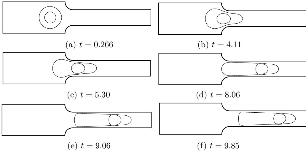
Figure 2: Snapshots of the transit of a compound drop into the capillary. Ca = 0.179 , Re = 1.56 \times 10^{-2} and \zeta_c = 0.72 . Time is scaled by a/V .
