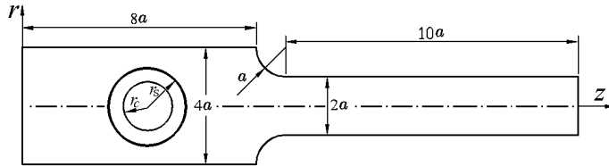
Figure 1: Geometric setup for simulating the deformation of a compound drop through a 2:1 contraction. Two cylindrical tubes are connected by an arc of radius a and central angle 90^\circ . Shown is the meridian plane and the upper half is the computational domain.
