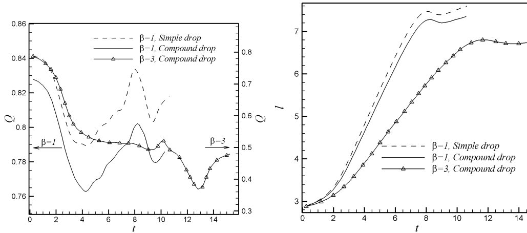
Figure 3: Temporal variations of the instantaneous flow rate Q and the length of the compound drop l for the process of Fig. 2. For comparison, we have also plotted results for a simple drop of the same size (radius 1.4a ) and fluid properties as well as for a compound drop with a more viscous shell ( \beta = 3 ).
