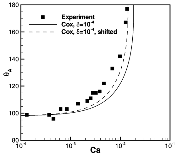
FIG. 3. Failure of the Cox formula to predict \theta_A(\text{Ca}) for liquid-liquid displacement in a capillary tube. The symbols are experimental data for a glycerin-silicone oil system with \theta_S=98^\circ and receding-to-advancing viscosity ratio \eta=0.9 . The solid line is the prediction of the Cox formula with \delta=l_s/W=10^{-4} , and the dashed line is the same prediction shifted to the left by multiplying Ca by a factor of 1.3 (or equivalently setting \delta=10^{-5.2} ). Adapted from M. Fermigier and P. Jenffer (Ref. 11).
