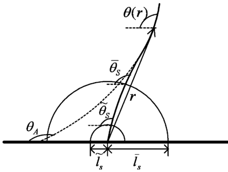
FIG. 6. Schematic illustrating the three contact angles \tilde{\theta}_s , \bar{\theta}_s , and \theta_A evaluated at different length scales \tilde{l}_s , \bar{l}_s , and W . Note that \theta_A is extracted from the static-like portion of the macroscopic interface.
