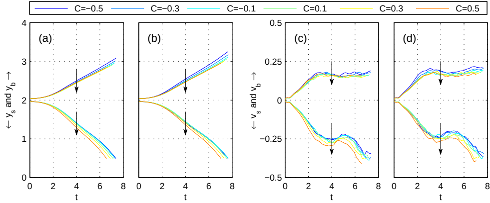
Figure 6: Spike and bubble tip position (a,b) and velocity (c,d) for \mathcal{P} = -0.3 (a,c) and \mathcal{P} = +0.3 (b,d); the arrow shows the direction of increasing \mathcal{C} .
