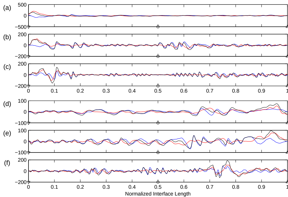
Figure 11: Electric force (red), surface tension (blue) and resultant contribution of interfacial forces (black) on vortex sheet strength in right hand side of equation (12); symbols on the horizontal axes correspond to spike tip ( \nabla ), middle point of interface ( \circ ) and bubble tip ( \triangle ). These symbols correspond to those in figure 10 on the interface. (a,b,c) NP with E_g = 5.625 at y_s = 1.7, 1.1 and 0.5 ; (d,e,f) PN with E_g = 5.625 at y_b = 2.1, 2.5 and 2.9 .
