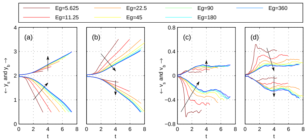
Figure 8: Spike and bubble tip position (a,b) and velocity (c,d) for NP ( \mathcal{P} = -0.3 - \mathcal{C} = +0.3 ) (a,c) and PN ( \mathcal{P} = +0.3 - \mathcal{C} = -0.3 ) (b,d); the arrows show the direction of increasing Eg (decreasing field intensity).
