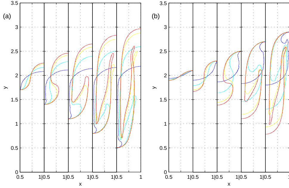
Figure 9: Interface profiles for E_g = 5.625 (blue), 22.5 (cyan), 90 (yellow) and 360 (red); (a) NP ( \mathcal{P} = -0.3 - \mathcal{C} = +0.3 ) at spike height y_s = 1.7, 1.4, 1.1, 0.8 and 0.5 ; (b) PN ( \mathcal{P} = +0.3 - \mathcal{C} = -0.3 ) at bubble height y_b = 2.1, 2.3, 2.5, 2.7 and 2.9 .
