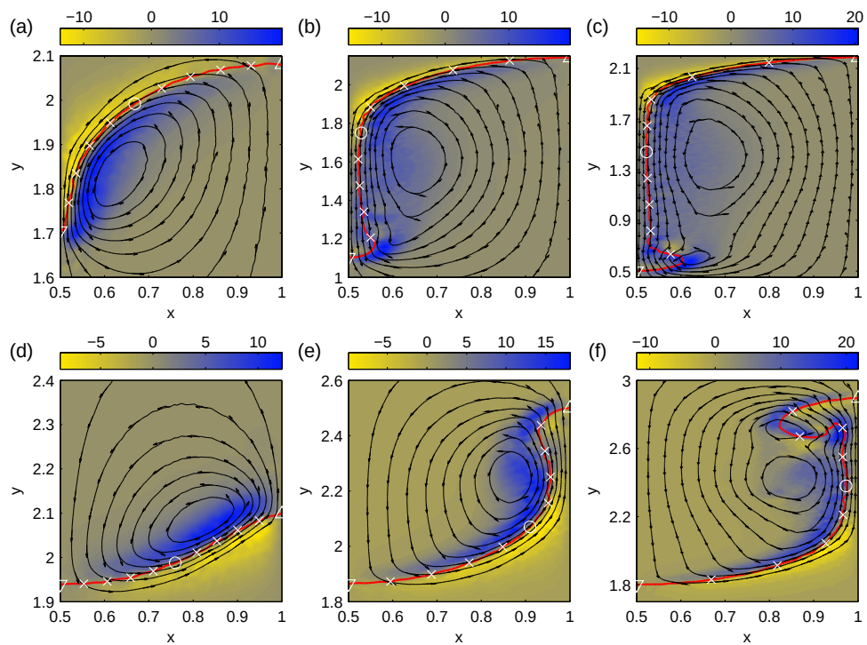
Figure 10: Contours of vorticity (fills) and streamlines (lines); the cross marks on the interface are placed at 0.1 intervals of normalized interface length. Symbols on the interface (figure 11 on the horizontal axes) correspond to spike tip ( \nabla ), middle point of interface ( \circ ) and bubble tip ( \triangle ). (a,b,c) NP with E_g = 5.625 at y_s = 1.7, 1.1 and 0.5 (blue contours in figure 9-a); (g,h,i) PN with E_g = 5.625 at y_b = 2.1, 2.5 and 2.9 (blue contours in figure 9-b).
