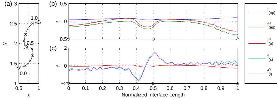
Figure 4: Profiles of normal force magnitudes along the interface for case PN; (a) interface profile; (b) electrical force and its components; (c) electrical force, surface tension and the resultant interfacial force; the cross marks on the interface are placed at 0.1 intervals of normalized interface length. Symbols on the interface and horizontal axes correspond to spike tip ( \nabla ), middle point of interface ( \circ ) and bubble tip ( \Delta ).
