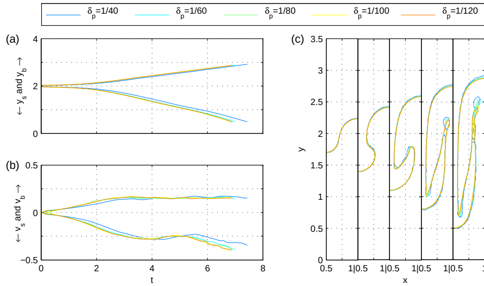
Figure 1: Spike and bubble tip positions (a) and velocities (b) versus time for different particle spacings of \delta_p = 1/40, 1/60, 1/80, 1/100 and 1/120 ; (c) interface profiles at y_s = 1.7, 1.4, 1.1, 0.8 and 0.5 .
