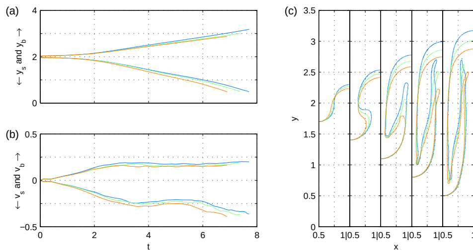
Figure 2: Spike and bubble tip positions (a) and velocities (b) for cases NP (red), PN (blue) and NE (green); (c) interface profiles at y_s = 1.7, 1.4, 1.1, 0.8 and 0.5 .
