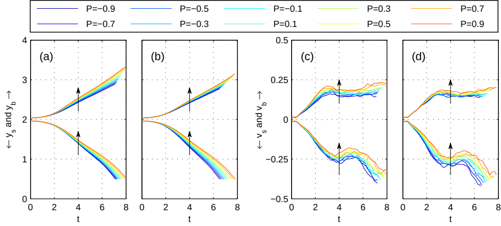
Figure 5: Spike and bubble tip position (a,b) and velocity (c,d) for C = -0.3 (a,c) and C = +0.3 (b,d); the arrow shows the direction of increasing \mathcal{P} .
