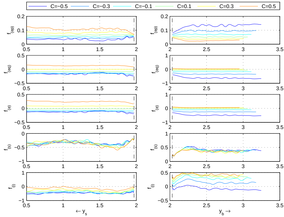
Figure 7: Magnitude of spike tip forces (left) and bubble tip forces (right) with respect to tip position for \mathcal{P} = +0.3 . The dash-dot line shows the starting position of the spike and bubble tip. f_{(e)} is the electric force (cf. equation (8)) while f_{(ep)} and f_{(eq)} denote polarization and Coulomb components of the electric force, respectively. f_{(s)} is the surface tension force (cf. equation (7)) and f_{(i)} is the resultant interfacial forces.
