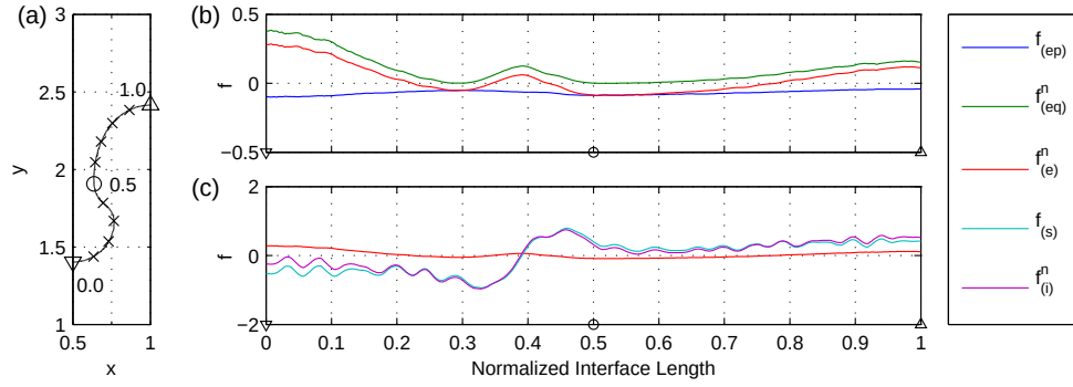
Figure 3: Profiles of normal force magnitudes along the interface for case NP; (a) interface profile; (b) electrical force and its components; (c) electrical force, surface tension and the resultant interfacial force; the cross marks on the interface are placed at 0.1 intervals of normalized interface length. Symbols on the interface and horizontal axes correspond to spike tip ( \nabla ), middle point of interface ( \circ ) and bubble tip ( \Delta ).
