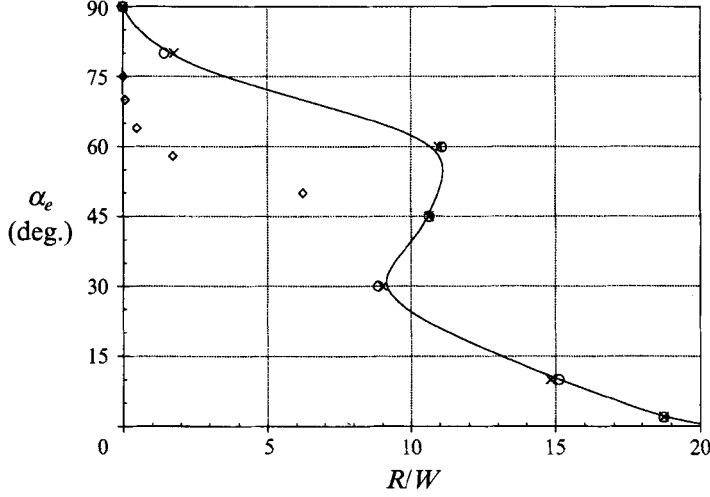
FIGURE 7. The equilibrium tilt angle as a function of the ratio of the Reynolds number to the Weissenberg number. This ratio is related to the climbing constant by R/W = 0.741\rho a^2/\beta . ○, Data points computed from (15) and the solid line is a smoothed curve-fitting to the circles; ×, data points obtained by neglecting the sidewise drift of the particle; ◇, experimental points from Liu & Joseph (1993) (the last point at R/W = 6.25 corresponds to R = 3.6 , which is out of the range of the perturbation theory).
