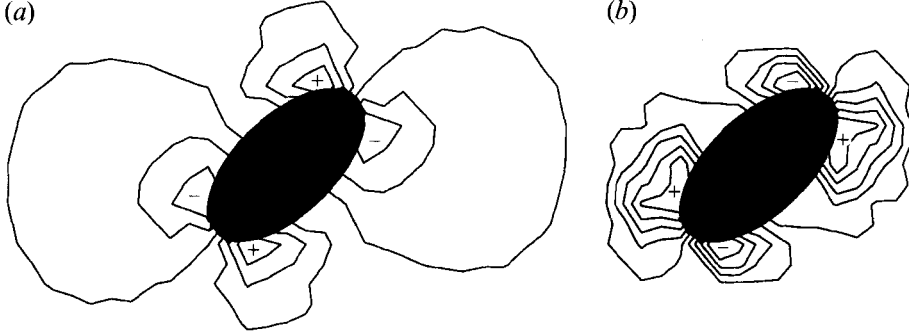
FIGURE 10. (a) Pressure contours on the symmetry plane due to inertial perturbation. The velocity field u_1 causes two high pressures (marked by 'plus' signs) and two low pressures (marked by 'minus' signs) on the surface of the ellipsoid which give rise to a negative torque. (b) Pressure contours on the symmetry plane due to normal stress perturbation. The velocity field u_2 causes two high pressures (marked by 'plus' signs) and two low pressures (marked by 'minus' signs) on the surface of the ellipsoid which give rise to a positive torque.
