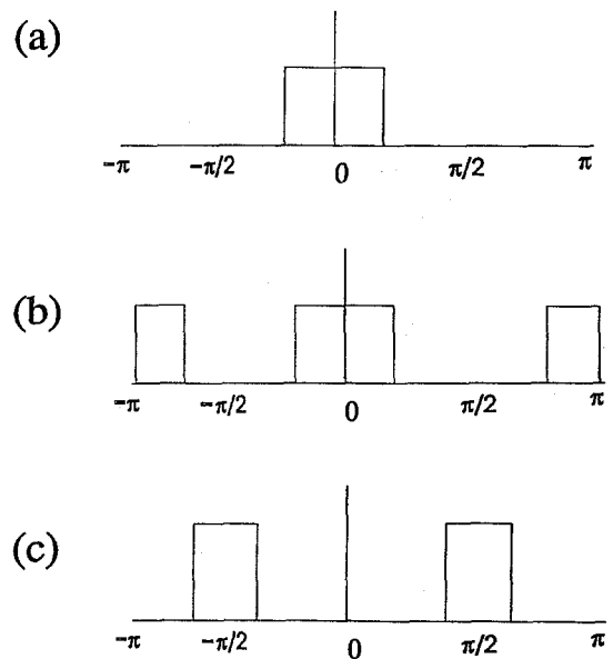
Fig. 3. The kernels K used to represent the contact alignment phenomena are shown here as functions of the angle between cells. (In 2D the angle is \theta , and in 3D it is \Omega .) (a) Single humped kernel, representing alignment in which both cells are oriented head-to-head. (b) Double humped kernel which permits cells to align also in a head-to-tail configuration. (c) An orthogonal interaction kernel that plays a role in the model for actin alignment.
