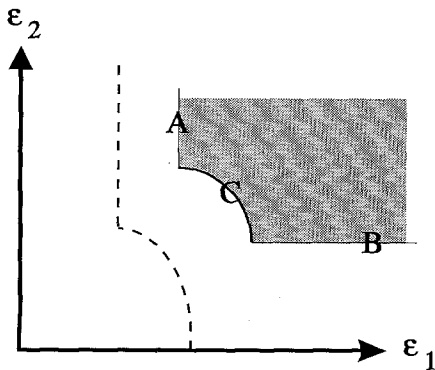
Fig. 6. The same as Fig. 4, but with an additional line for primary bifurcation (C). This line corresponds to the growing mode n \neq 0 , q \neq 0 .
