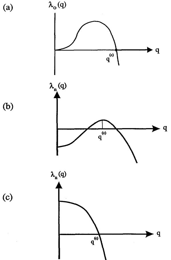
Fig. 9. The linear growth rate of an unstable mode as a function of q . (a) and (c) correspond to Figs. 8a,c respectively. (b) corresponds to Fig. 8a if \epsilon_2 is large, and to Fig. 8b if \epsilon_2 is small.
