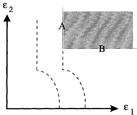
Fig. 4. A complete bifurcation diagram. A and B are the lines of primary bifurcations. Line A corresponds to the growing mode n \neq 0 , q = 0 . Line B corresponds to n = 0 , q \approx 0 . The shaded region is the region of stability of the homogeneous state. The unshaded region corresponds to some non-homogeneous pattern. The dashed lines are secondary bifurcations. The vertical dashed lines correspond to n \neq 0 , q \neq 0 . The curved portion of the dashed lines corresponds to n \neq 0 , q \neq 0 .
