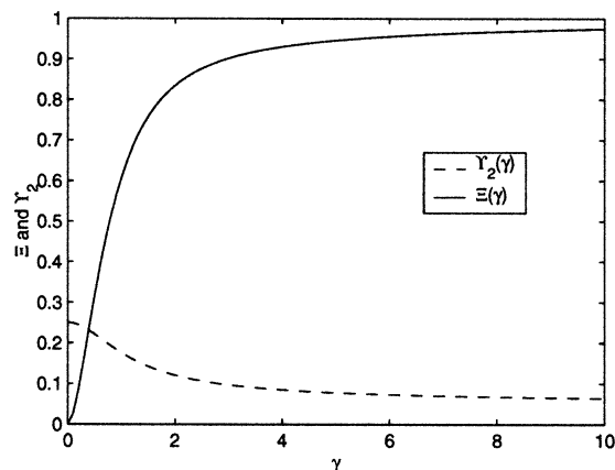
FIG. 7. The solid curve is the function \Xi(\gamma) \equiv 4\pi \sum_{n=1}^{\infty} n I_n^2(\gamma) in (56) and (57). The dashed curve is the function \gamma_2(\gamma) defined in the discussion surrounding (60).
