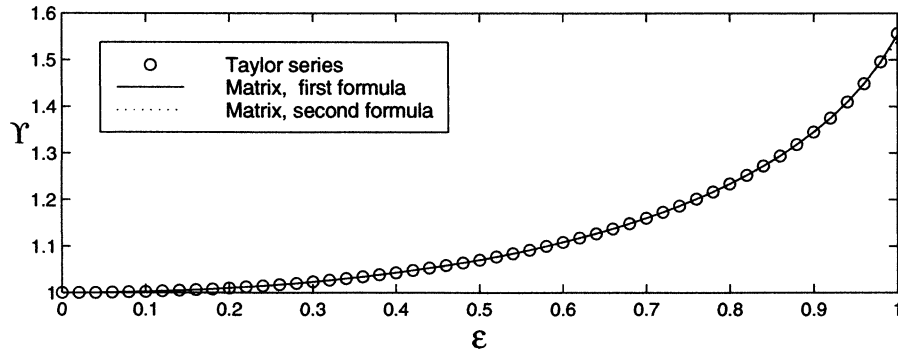
FIG. 2. Function Y(\epsilon) computed using three different methods. The Taylor series method uses 61 terms in the series (44). The first matrix formula uses the series in (40) and the second matrix formula uses the series in (41). The three methods agree to within the linewidth of the graphs.
