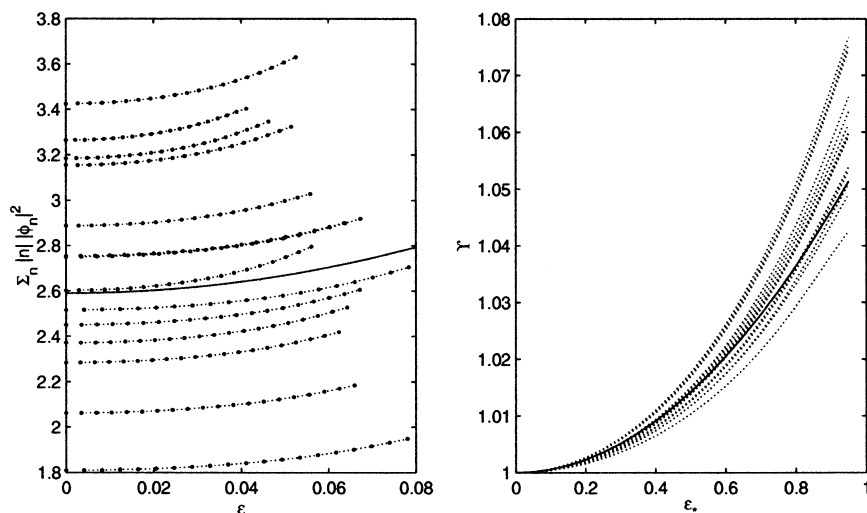
FIG. 12. (left) The 14 dashed curves show the sum \Gamma(\epsilon) in (67) calculated using 14 realizations of the topography. The maximum slope, S_{\max}^x , was typically of order 15 and so \epsilon_* = 0.95 corresponds to maximum values of \epsilon of about 0.06. (right) The enhancement factor for the 14 topographies, Y(\chi, \epsilon_*^x) \equiv \Gamma(\epsilon, \chi)/\Gamma(0, \chi) . In the right panel, the rescaled parameter \epsilon_*^x defined in (66) is used as the abscissa. In both panels, the solid curve shows the results expected from the small- \epsilon perturbation theory.
