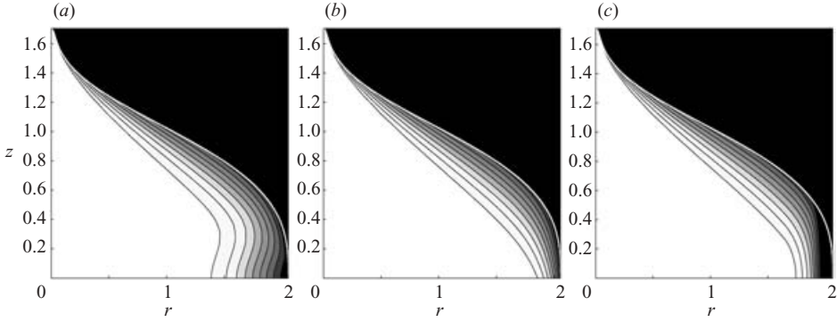
FIGURE 8. A comparison of the height and temperature fields at t=11 for a dome with \kappa=0.01 , and \gamma=B=0 . The panels show isotherms (spaced by 0.1 from 0 (black) to 1 (white)). Panel (a) shows the full numerical solution, (b) displays the profile computed from the surface temperature assuming the integral-balance ansatz for the temperature field ( \Theta = \Theta_b - (\Theta_b - \Theta_s)(1 - (h - z)/\delta)^2 , where \delta = \text{Min}[2\kappa^{1/2}(1 - \Theta_s)/\Theta_s, h] and \Theta_b = \Theta_s(\delta + 2\sqrt{\kappa})/(2\sqrt{\kappa}) ), and (c) shows the integral-balance solution computed using the skin theory of §4.
