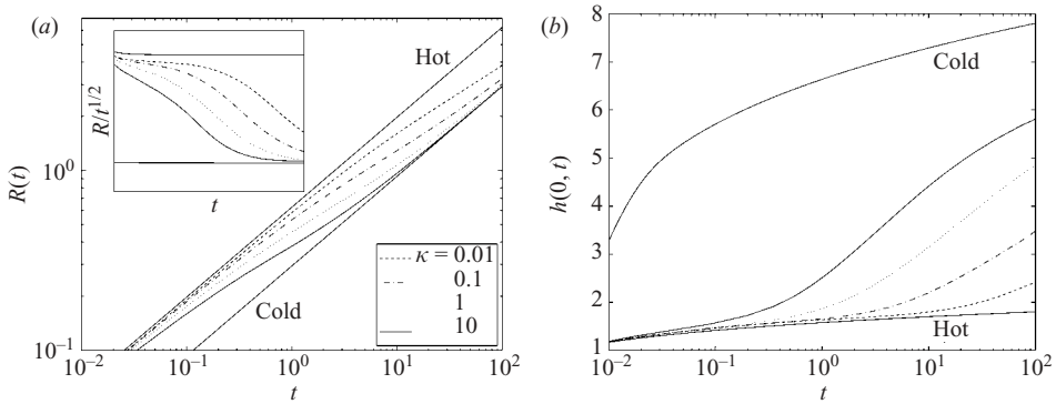
FIGURE 3. (a) Dome radius and (b) maximal height for the computations of figure 1. B = 0 , \gamma = 6 . The solid curves marked hot and cold show isothermal extrusions for fluids at the eruption and ambient temperatures. The trends of the expected power laws for an isothermal Newtonian fluid are h(0, t) \sim t^0 and R(t) \sim t^{1/2} ; the inset in (a) shows R(t)/t^{1/2} versus t .
