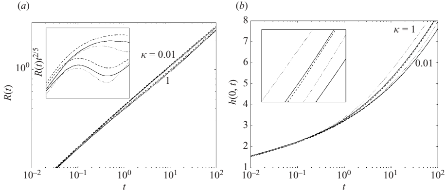
FIGURE 12. (a) Dome radius and (b) maximal height for two of the computations of figure 10 with \kappa = 0.01 and 1, and B = 10 and \gamma = 6 . The dashed lines show the skin model. The results of the full thin-layer model are represented by solid lines. The vertically isothermal model is represented by dotted lines. The inset in (a) shows the data replotted as R/t^{2/5} ; the inset in (b) shows a magnification near t = 100 . In (b), the full thin-layer model and skin theory are indistinguishable.
