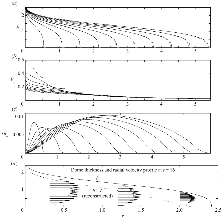
FIGURE 14. A simulation where the surface viscosity is relatively large and the velocity field in the skin becomes practically zero. a_0 = 2 and \gamma = 6 ; \delta is constructed assuming \kappa = 10^{-3} , but is not included in the computation and here simply shows where the skin would have been as a consistency check. The dotted lines in (a) show an isothermal simulation constrained to have a surface on which u = 0 and can only be lifted vertically.
