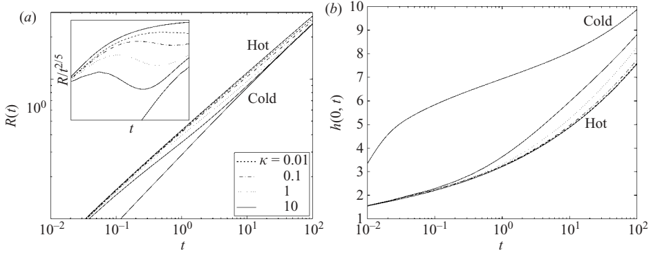
FIGURE 6. (a) Dome radius and (b) maximal height vs. time for B = 10 , \gamma = 6 and four values of \kappa . The curves marked hot and cold show isothermal extrusions for fluids at the eruption and ambient temperatures. For an isothermal yield-stress-dominated dome we expect R(t) \sim t^{2/5} ; in (a), the inset replots the data as R/t^{2/5} versus t .
