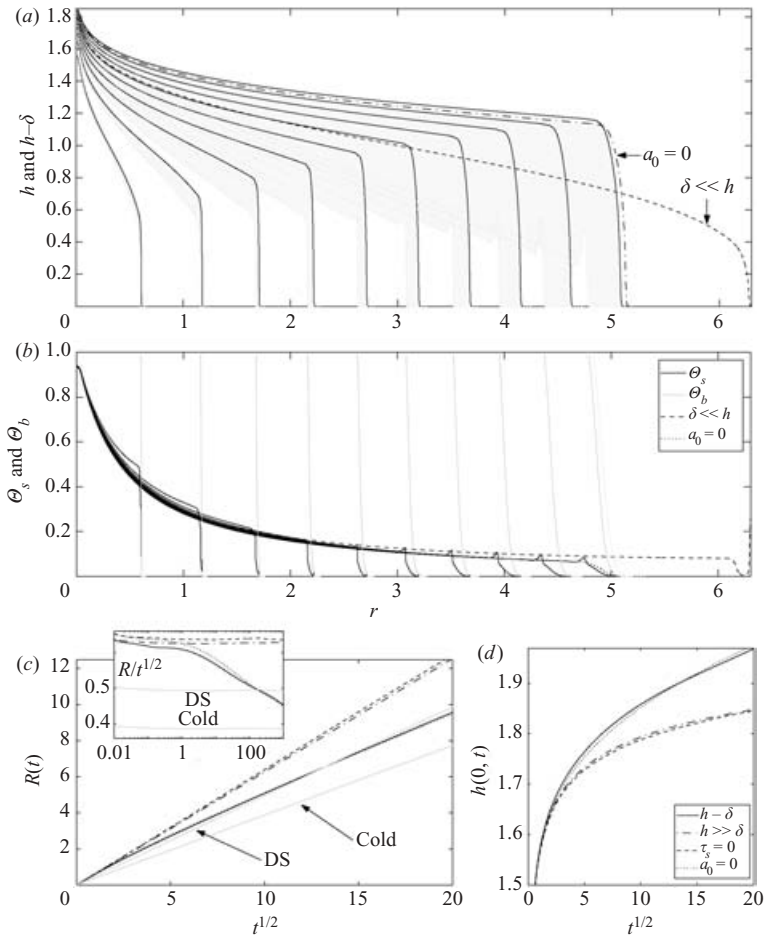
FIGURE 17. An extrusion with small extensional stress and finite skin thickness. (a) Snapshots of the dome surface and skin for t=n^2 and n=1, 2, \dots, 10 ; the shaded region shows the skin. The dashed curve shows the final height profile if the skin thickness were assumed infinitely thin, and the dash-dotted line shows an extrusion assuming a_0=0 . (b) shows corresponding surface and basal temperatures, \theta_s and \theta_b . (c, d) show the dome radius and maximal height against time. Also displayed are the radius and height for an isothermal extrusion with stress-free surface (labelled \tau_s=0 ), the extrusion with a_0=0 , an extrusion with a cooling skin assuming \delta \ll h . In (c), showing the evolution of the dome radius, we have added two extra curves (by light solid lines); these show the radius of a dome expanding isothermally at the ambient temperature ('Cold'), and the prediction expected from dimensional scaling ('DS'), assuming that a slender edge controls the expansion (see §4.1). \kappa=10^{-3} , \gamma=4 , a_0=10^{-4} .
