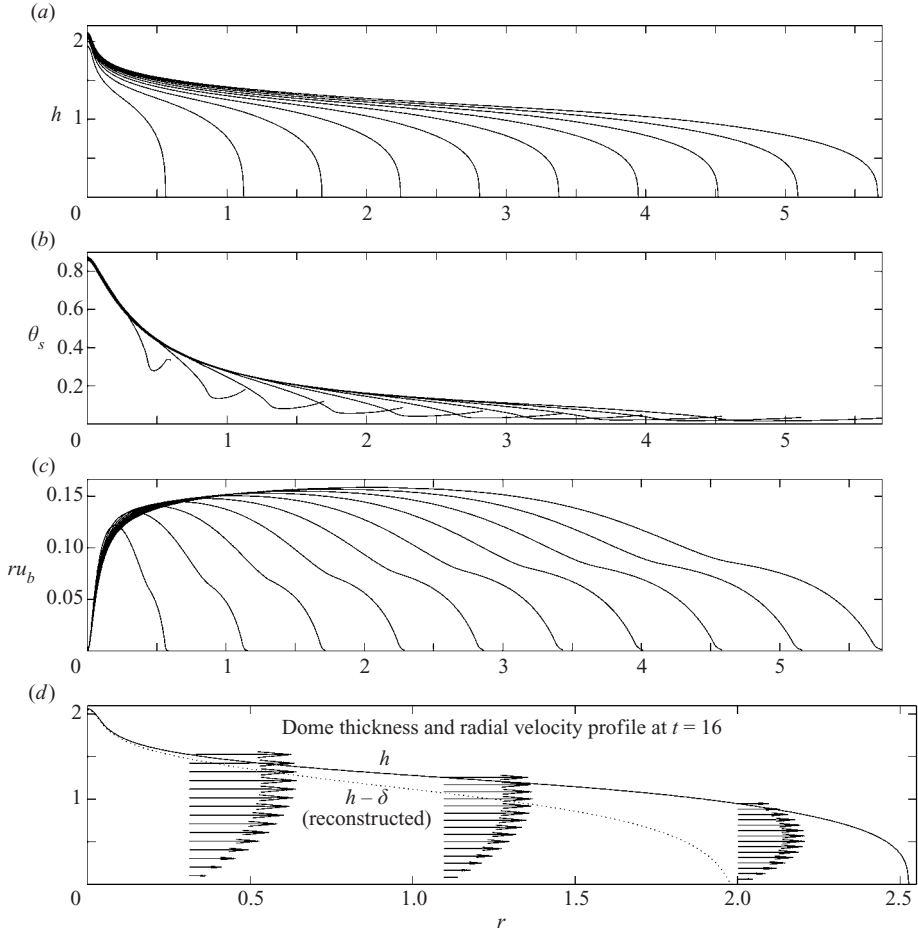
FIGURE 15. Sample solution for a source with intermediate skin strength. (a)–(d) as in figures 13–14. a_0 = 0.05 , \gamma = 4 and \kappa = 10^{-3} .
