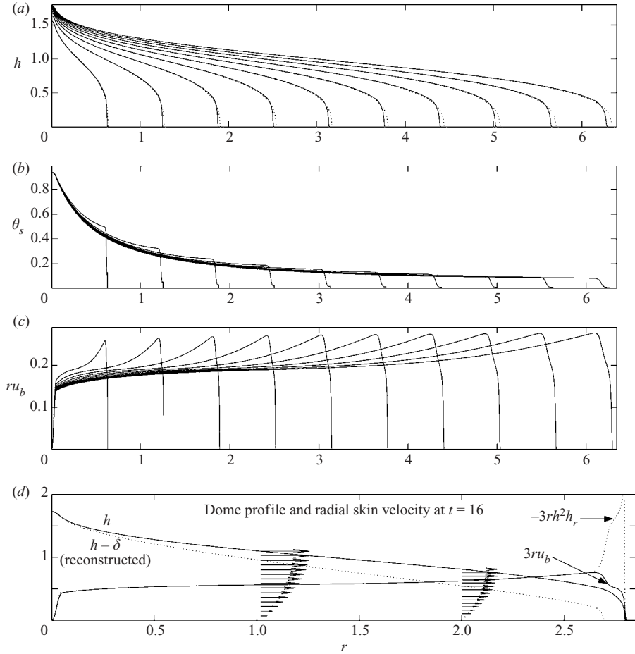
FIGURE 13. A simulation for a source with B=0 , assuming the thermal boundary layer has negligible thickness ( \delta \ll h ). (a)–(c) show snapshots of the thickness, the surface temperature and ru_b at the times t = n^2 , n = 1, 2, \dots, 10 . The dotted lines in (a) show the corresponding isothermal solution with a free surface. In this case, the surface viscosity is not large and the surface velocity field approaches -h^2h_r/2 (the usual isothermal result) except for boundary layers at the source and near the edge, as shown in (d). This picture also shows the extent of the skin at t = 16 , had it not been assumed infinitesimally thin (hence displaying a consistency check), and illustrates the vertical profile of the radial velocity. The parameters of the model are a_0 = 10^{-4} and \gamma = 4 . The diffusion parameter \kappa does not appear explicitly in the theory when \delta is assumed much less than h ; in (d), \delta is reconstructed assuming \kappa = 10^{-3} .
