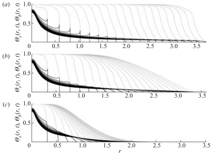
FIGURE 7. Snapshots of the surface and basal temperature profiles for three computations with \gamma = 6 and B = 10 . Times are t = 0.55n^2 , n = 1, 2, \dots, 20 . The darker lines show the surface temperature, whereas the lighter lines show the basal temperature. (a) \kappa = 0.01 , (b) 0.1, (c) 1.
