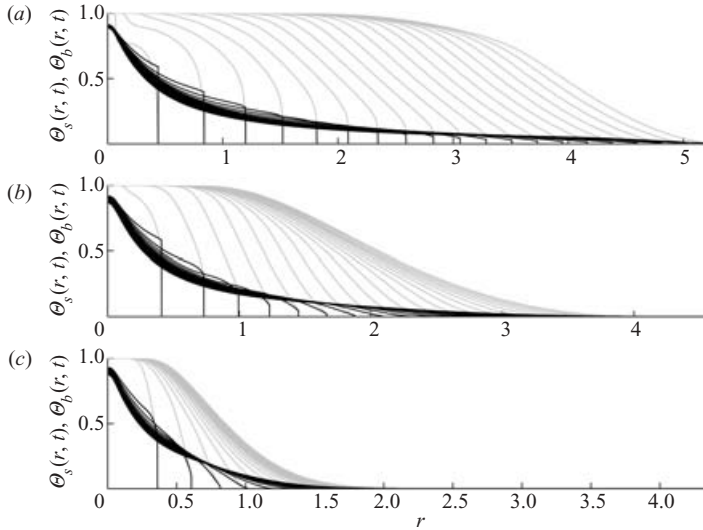
FIGURE 4. Snapshots of the surface and basal temperature profiles for three of the computations of figure 1. Times are t = 0.55n^2 , n = 1, 2, \dots, 20 . The darker lines show the surface temperature, whereas the lighter lines show the basal temperature. (a) \kappa = 0.01 , (b) 0.1, (c) 1.
