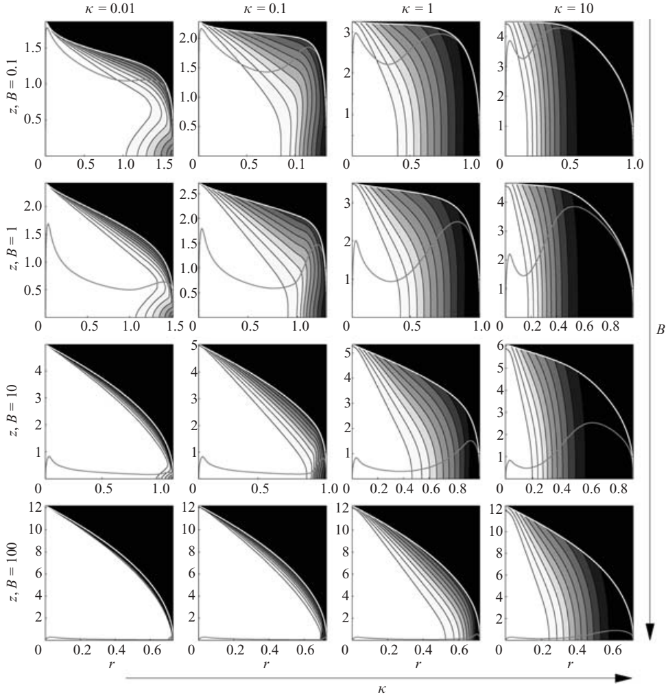
FIGURE 5. Snapshots at t = 11 for four numerical computations with \gamma = 6 and differing \kappa and B . As in figure 1, each picture shows isotherms. Also shown by the lighter solid curve is the fake yield surface, z = Y(r, t) . Each column represents a computation with different inverse Péclet number: \kappa = 0.01, 0.1, 1 and 10 . Each row represents a different B : 0.1, 1, 10 and 100 .
