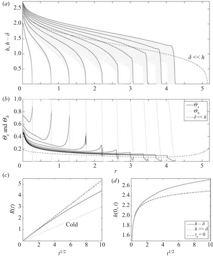
FIGURE 18. A similar picture to figure 17 showing an extrusion with a strong extensional stress and finite skin thickness. In this case, neither the extrusion with a_0 = 0 nor the dimensional scaling result are shown. \kappa = 10^{-3} , \gamma = 4 , a_0 = 2 .
