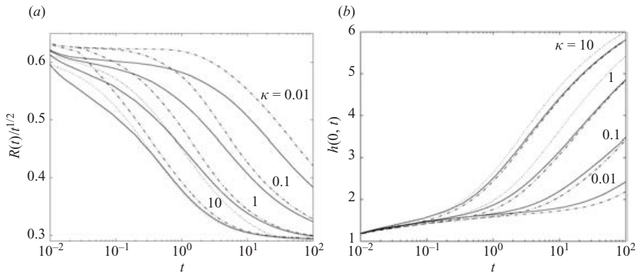
FIGURE 11. (a) Dome radius and (b) maximal height for the computations of figure 10 with B=0 and \gamma=6 . The dashed lines show the skin model. The results of the full thin-layer model are represented by solid lines; the results of the vertically isothermal model are shown by dotted lines; only \kappa=1 and 10 are displayed since the others are too discordant to display.
