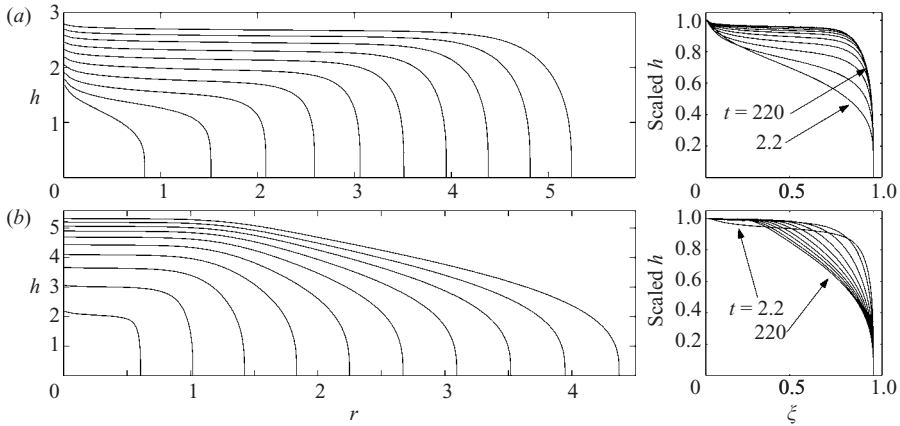
FIGURE 2. Snapshots of the dome thickness at the times t = 2.2n^2 , n = 1, 2, \dots, 10 for (a) \kappa = 0.01 and (b) \kappa = 1 , with B = 0 and \gamma = 6 . The data are redrawn, scaling radius by the dome radius, \xi = r/R , and thickness by dome height, h(r, t)/h(0, t) , in the two smaller panels.
