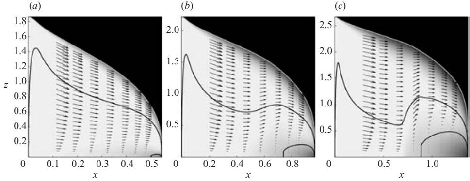
FIGURE 19. Snapshots of an evolving dome with a temperature-dependent yield stress at times (a) t = 1 , (b) 4 and (c) 11, of the temperature distribution (colourmap), the fluid surface (lighter lines) and fake yield surfaces (dark lines). The yield stress is given by \tau_p(T) = \tau_p(T_e)e^{\gamma_B(1-\Theta)} , with \gamma_B = 6 and B = H\tau_p(T_e)/(\eta_e U) = 1 . The other parameters were \gamma = 6 and \kappa = 0.01 . More details of the numerical procedure are given in Appendix A.2.
