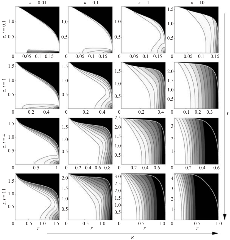
FIGURE 1. Snapshots of evolving domes: Four numerical computations with \gamma = 6 and B = 0 . Shown are contours of constant temperature on the (r, z) -plane; contours are spaced by 0.1, from 0 (black: cold) to 1 (white: hot). Each column represents a computation with different inverse Péclet number: \kappa = 0.01, 0.1, 1 and 10. Each row represents a snapshot at a given time: t = 0.1, 1, 4 and 11.
