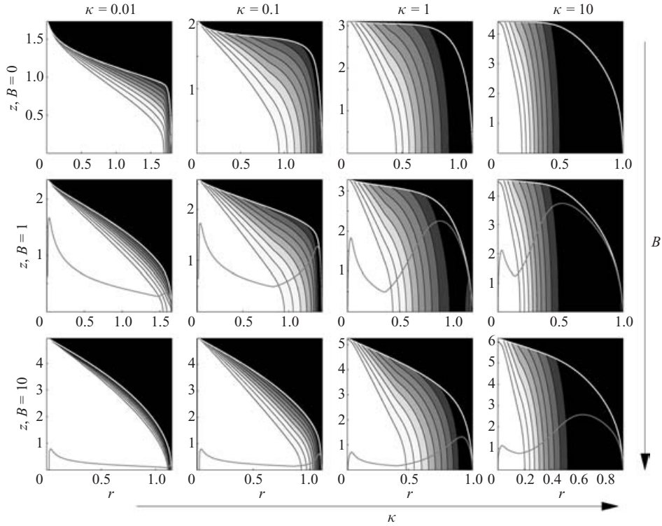
FIGURE 10. Snapshots of numerical solutions of the skin theory for B=0, 1 and 10 , with \kappa=0.01, 0.1, 1 and 10 at t=11 . The three rows should be compared with corresponding rows in figures 1 and 5.
