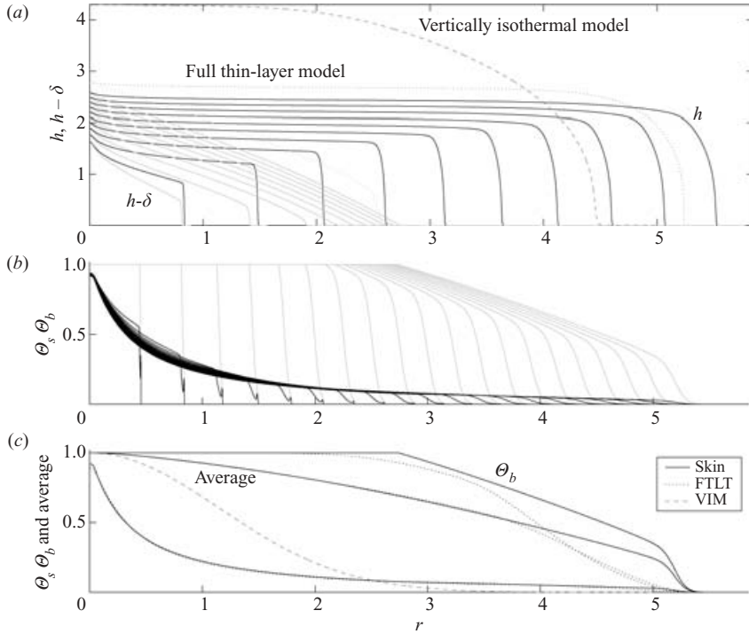
FIGURE 9. A solution of the skin model with B=0, \kappa=0.01 . The panels show snapshots of (a) thickness (dark lines) and skin depth h - \delta (light lines), and (b) surface (dark lines) and basal (light lines) temperature at t = 2.2n^2 , n = 1, \dots, 10 . In (a), we also show the final thickness profiles of the full thin-layer theory (FTLT) and the vertically isothermal model (VIM), together the \Theta = 0.95 isotherm of the full theory (light dotted line; this isotherm provides an estimate of skin depth). Panel (c) compares the final temperature distributions of the three models (namely the surface, basal and vertically averaged temperatures). The surface temperatures of the skin model and full thin-layer theory are barely distinguishable, whereas the vertically isothermal model only provides a prediction of the average.
