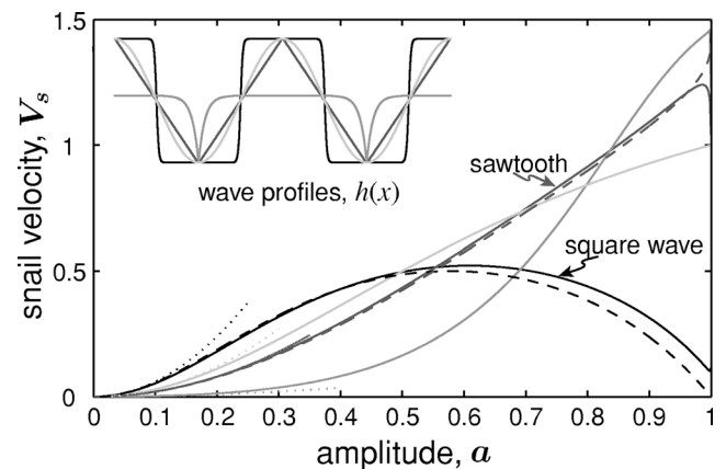
FIG. 12. Dimensionless snail speeds for different wave profiles. The square-wave-like profile is given by \delta=\tanh 12 \cos(2\pi x) , and the sawtooth-like profile by a Fourier series truncated at 16 terms. The spiky, sharp profile was built using the function \exp(-6\sqrt{1+\cos 2\pi x}) . The dotted lines show the initial parabolic behavior; the dashed lines show the sawtooth and square wave snail velocity as a function of wave amplitude.
