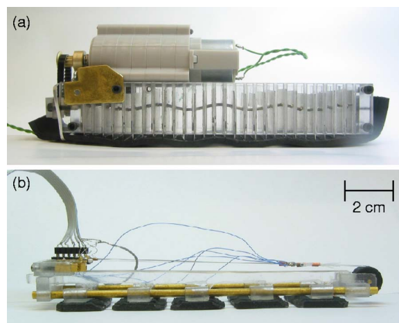
FIG. 2. (Color online). Photograph of two prototype mechanical crawlers. (a) Retrograde crawler (details in Sec. III A). (b) Direct crawler (details in Sec. III B). The direct crawling device is capable of climbing a vertical wall and performing an inverted traverse.
