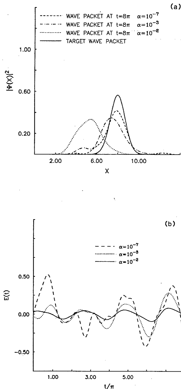
FIG. 3. Three distinct wave packets, each corresponding to different values of \alpha . The parameter \alpha determines the relative importance between the term that represents error in achieving the target state \hat{\psi} , and the magnitude of the applied potential. In each case a spatially constrained applied potential of the form -(X-4)E(t) is sought. (a) The probability densities at time T=8\pi of the three wave packets and that of the target. Initially \psi_0(X)=g(X,4,1) and the final target at time T is \hat{\psi}(X)=g(X,8,1) for each of the wave packets. (b) The applied electric field E(t) for each of the values of \alpha . As \alpha is increased the magnitude of the applied field is restricted, which limits the extent to which the target state \hat{\psi} can be achieved as can be seen in (a). As a result of an increase in \alpha the applied field E(t) also loses some of the important phase adjustment structure as can be seen clearly in the early time interval [0,4\pi] upon comparison of the cases \alpha=10^{-3} and 10^{-7} in (b). All the quantities used in this figure are dimensionless.
