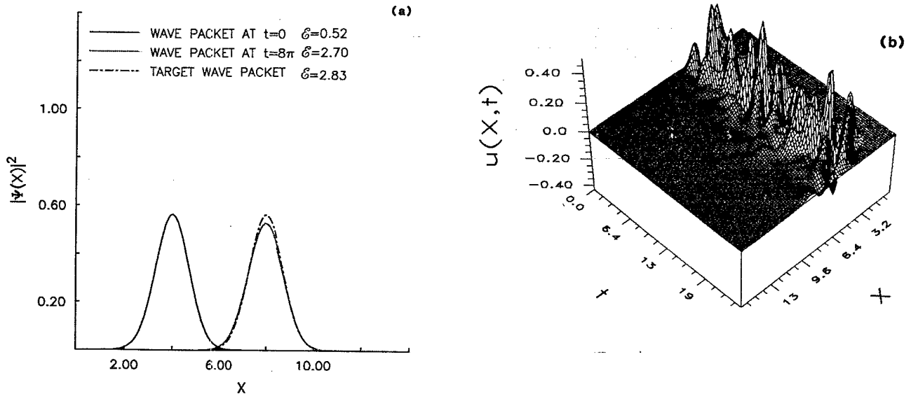
FIG. 2. A Gaussian wave packet translated from X_0 = 4.0 to X_f = 8.0 by an unconstrained applied potential (P2) u(X, t) . (a) The probability densities of the initial wave packet \psi_0(X) , the final wave packet \psi(X, T) achieved using u(X, t) , and the target wave packet \hat{\psi}(X) . (b) The external applied potential u(X, t) over the space-time domain [0, 16.0] \times [0, 8\pi] . The spatially localized, complex structure of this potential should be contrasted with that of the constrained potential shown in Fig. 1(b). (c) Three space-time plots with an aligned time interval. (i) Regions of positive (dark shading) and negative (light shading) applied potential u(X, t) . (ii) A contour plot of the probability density |\psi(X, t)|^2 with contour intervals \Delta |\psi|^2 = 0.1 . (iii) Positive and/or negative regions of the flux vector J(X, t) . The positive regions (dark shading) represent regions in which there is a flux of material in the positive- X direction, whereas negative regions (light shading) represent regions in which the flux of material is in the negative- X direction. A similar period to that of Fig. 1 of high-frequency phase adjustment can be observed. This is followed by a stage in which the wave packet is guided to the objective by a deepening well indicated by the dashed line. The same dashed line on the contour plot of the probability density demonstrates the phase lag of the wave packet behind the external excitation. The large uninterrupted regions of material flux confirm that the wave packet is being channelled to the final state toward the end of the interval [0, 8\pi] . (d) The energy \mathcal{E}(t) of the wave packet over the time interval [0, 8\pi] . In this case the energy absorption of the wave packet is monotonic, which was not the case for the spatially constrained controller [see Fig. 1(f)]. All the quantities used in this figure are dimensionless.
