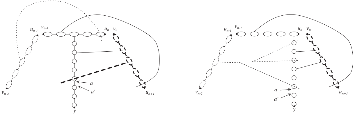
Figure 3: Two examples of the choice of cutting bond (a', a) . Solid lines represent C_n , dashed lines represent C_{n-1} , and bold dashed lines represent C_{n+1} .
