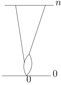
Figure 4: Schematic depiction of disjoint connections required by \Psi_n^{(1)} .
