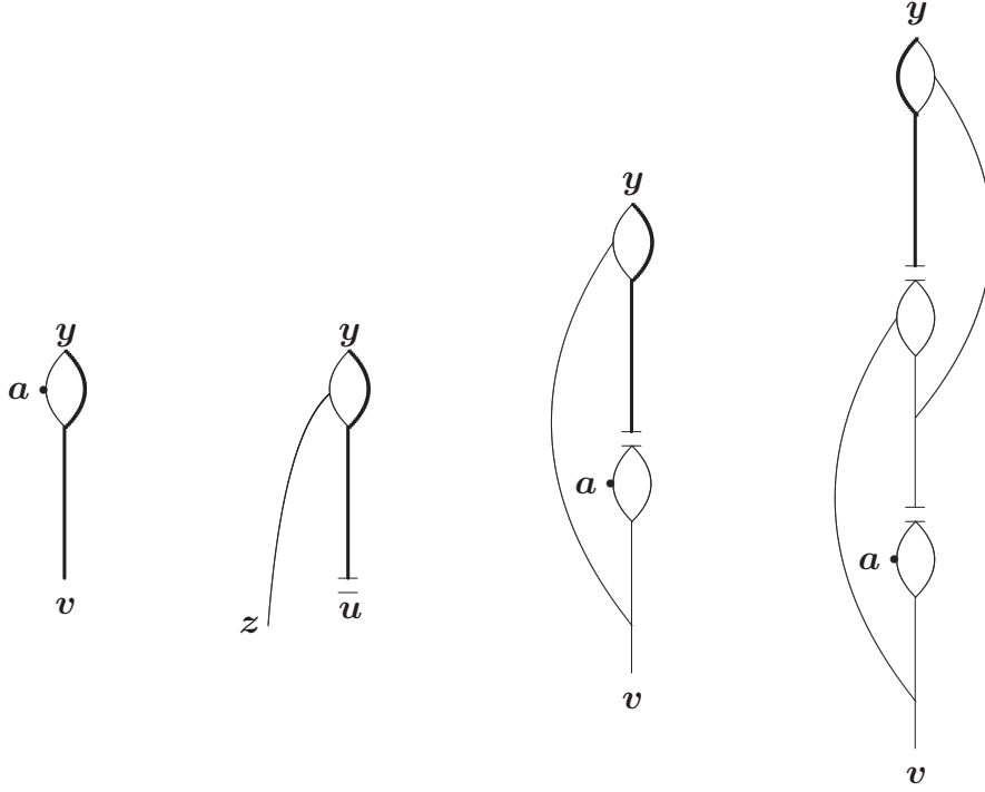
Figure 7: Diagrams for P^{(0)}(\mathbf{v}, \mathbf{y}; \mathbf{a}) , P(\mathbf{u}, \mathbf{z}, \mathbf{y}) , and examples of diagrams that contribute to P^{(1)}(\mathbf{v}, \mathbf{y}; \mathbf{a}) , P^{(2)}(\mathbf{v}, \mathbf{y}; \mathbf{a}) . The N -admissible lines are shown in bold.
