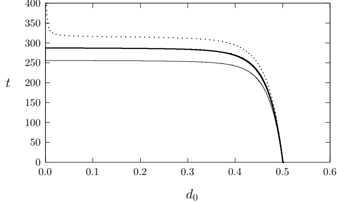
FIGURE 4. The distance d_0(t) of the flame-front tip to the boundary, from the numerical solution of the full PDE (1.8) (dashed line) and the solution of the asymptotic ODE (4.20) (solid line). The domain is the square \Omega = [0, 3] \times [0, 3] and \varepsilon = 0.113 . The heavy-solid line is the improved ODE (4.21) suggested by the one-dimensional theory.
