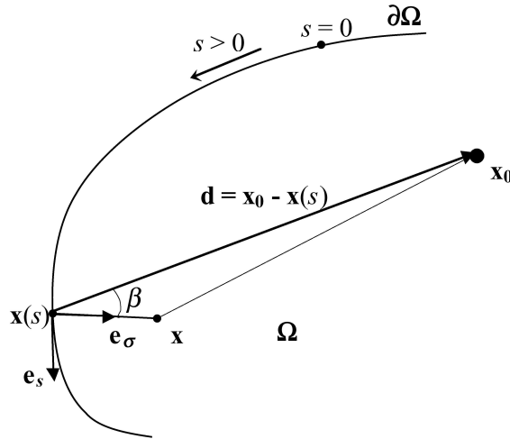
FIGURE 3. Coordinate system for the boundary layer analysis
