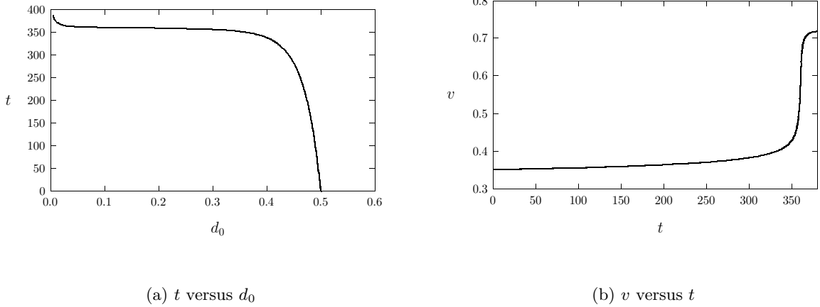
FIGURE 5. Numerical solution of (4.22) with \varepsilon = 0.11 for the flame-front tip in the unit disk. Left figure: the distance d_0(t) of the flame-front tip to the boundary. Right figure: the speed v(t) of the flame-front.
