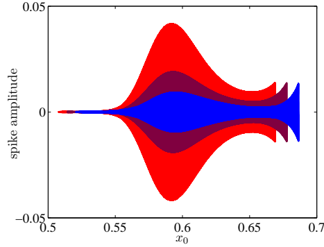
Figure 14: Plots of spike amplitude versus x_0 with (p, q, r, s) = (3, 3, 3, 0) , \varepsilon = 0.005 , D = 1 , and \tau = 1.245 . The three colors differ only in the starting location x_0(0) . In the red plot, starting closest to the bifurcation threshold, oscillations grow in the unstable regime to beyond their original value. In this case, the Hopf bifurcation is fully realized before the spike passes through the unstable zone. The purple plot shows that starting farther into the stable zone reduces the maximum oscillation amplitude attained in the unstable zone. Starting even farther back, the blue plot shows that the spike may pass safely through the unstable zone without the oscillation amplitude ever reaching its original value.
