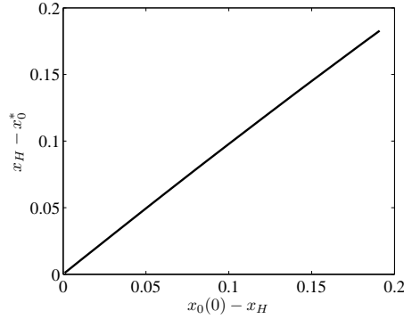
Figure 10: A plot of delay, x_H - x_0^* , versus the ‘‘initial buffer,’’ x_0(0) - x_H , where x_0(0) is the initial location of the spike, x_H is the Hopf bifurcation value, and x_0^* is the spike location at which the oscillation amplitude recovers to the size of the original perturbation. The exponents ((p, q, r, s) = (3, 3, 3, 0)) and value of D ( D = 4 ) correspond to the monotonic \tau_H(x_0) depicted in Figure 3(a), while \tau is set at 0.891.
