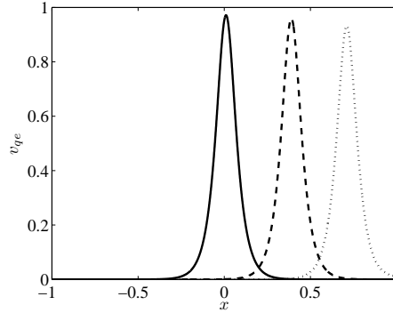
Figure 9: Plots of v_{qe} at various times during its evolution according to (3.9). The spike increases in height as it drifts toward x_0 = 0 . The parameters are (p, q, r, s) = (3, 3, 3, 0) , \varepsilon = 0.05 , D = 4 , and \tau = 0.01 . By Figure 3(a), this value of \tau is well below threshold for all x_0 , and so no oscillations in spike amplitude are present. The times depicted are t = 0 (dotted), t = 400 (dashed), and t = 2800 (solid).
