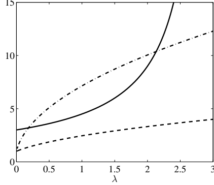
Figure 6: The function \mathcal{G}(\lambda) in (2.7) is indicated by the solid curve on the interval [0, 3] . The dashed curve depicts the function \sqrt{1 + \tau\lambda} for \tau sufficiently small so that it does not intersect \mathcal{G}(\lambda) . The dash-dotted curve depicts \sqrt{1 + \tau\lambda} for large \tau . In this case, there are two intersections, representing two positive real roots of (2.8).
