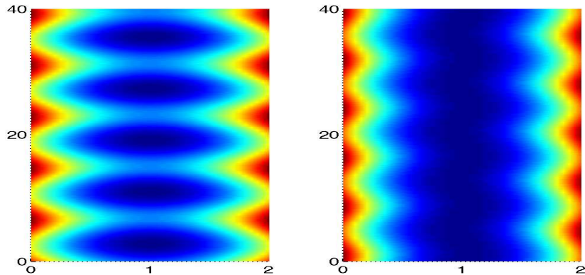
Figure 5: Full numerical solutions of the PDE-ODE system (2.1) demonstrating either in-phase or anti-phase oscillations of the two compartments. Time increases from bottom to top and the horizontal axis indicate the bulk region where L = 1 . Left panel: in-phase oscillations for D = 1 and \beta = 0.7 (solid dot in Fig 1). Right panel: anti-phase oscillations for D = 0.4 and \beta = 0.5 (open circle in Fig. 1.) The other parameter values are the same as in the caption of Fig.1.
