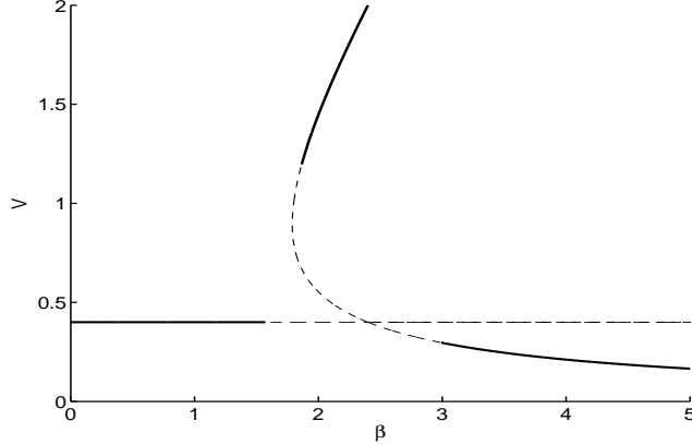
Figure 10: Bifurcation diagram of the ODE system (4.6) versus \beta for the parameter set \epsilon = 0.15 , \mu = 0.4 , \alpha = 0.55 , and L_v = 0.8 . The solid/dashed line represents stable/unstable steady-state solutions of V .
