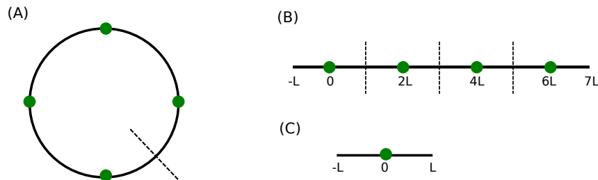
Figure 11: Left panel: Schematic diagram of four identical cells on a ring structure. The green solid dots represent cells. Top right panel: Schematic diagram of four identical cells on the domain [-L, 7L] with periodic boundary conditions at the two ends. Bottom right panel: schematic of one cell on [-L, L] centered at x = 0 .
