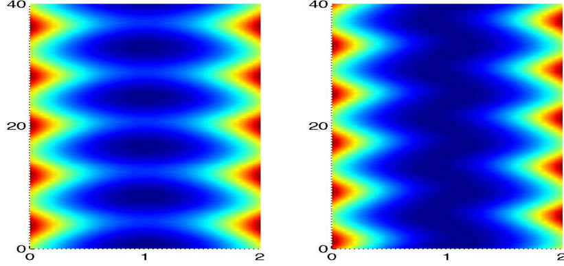
Figure 6: Full numerical solutions of the PDE-ODE system (2.1) for D = 0.4 and \beta = 0.8 , showing different long-time results depending on the initial conditions. Left panel: for the initial values C(x, 0) = 0.5 , v_1 = 0.3 , w_1 = 0.2 , v_2 = 0.4 , and w_2 = 0.2 , there are in-phase oscillations. Right panel: with the same initial values, but with v_1 = 5 and w_1 = 10 , we get anti-phase oscillations.
