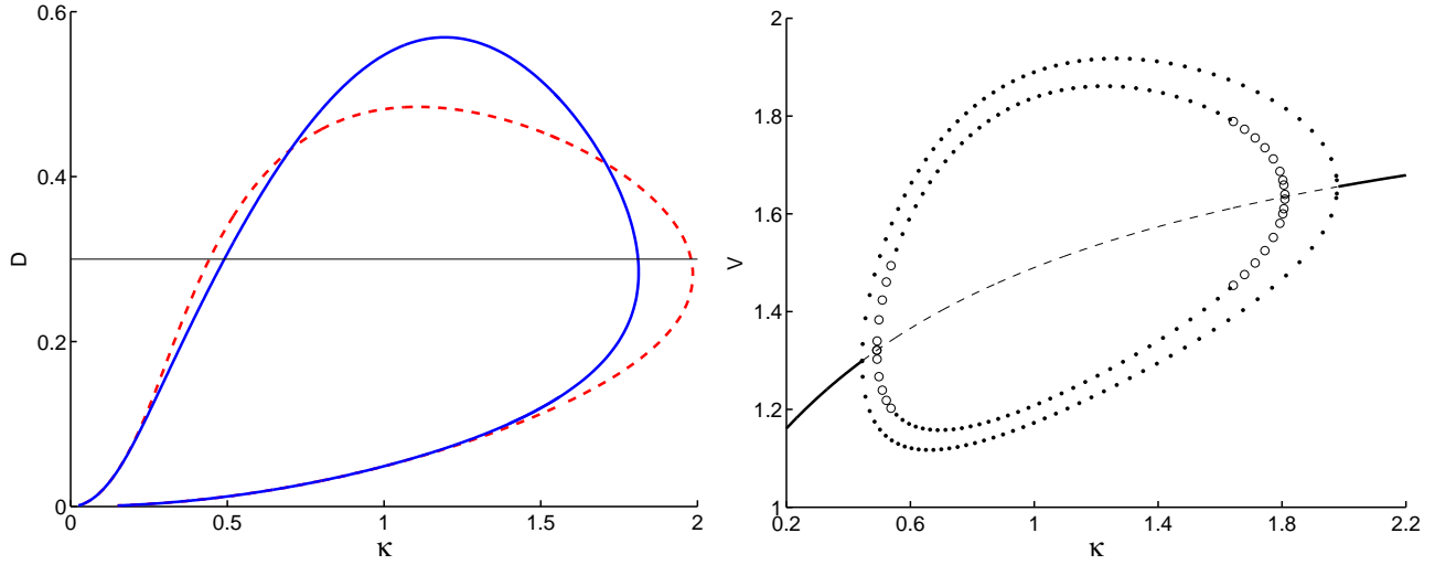
Figure 4: Left panel: Phase diagram in the D versus \kappa plane for \beta = 1 . The instability regions for in-phase and anti-phase compartmental oscillations are inside the solid and dashed curves, respectively. Right panel: Bifurcation diagram of V for the horizontal slice at D = 0.3 through the D - \kappa phase plane (see left panel) computed using XPPAUT [7]. The solid and dashed lines denote the linearly stable and unstable branches of steady-state solutions, respectively. The outer/inner closed loops correspond to branches of anti-phase/in-phase periodic solutions, where solid/open circles represent linearly stable/unstable periodic solutions. The other parameters are as in the caption of Fig. 1.
