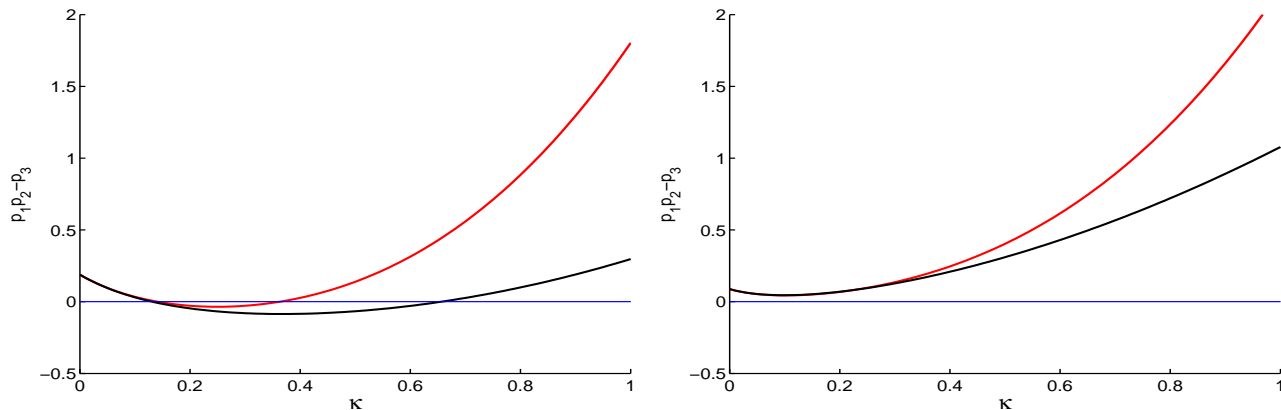
Figure 15: Plot of p_1 p_2 - p_3 versus \kappa for l = 0 (lower curve) and l = 1 (upper curve) for a ring of m = 3 cells. The horizontal line is the threshold p_1 p_2 = p_3 . Any intersections of the lower (upper) curves with the horizontal line yields the bifurcation points for \kappa for l = 0 ( l = 1 ). Left panel: the parameter values as given in Fig. 12. Between the two bifurcation points, the lower (upper) curve lies below the threshold p_1 p_2 = p_3 , and so by the Routh-Hurwitz criterion there are unstable eigenvalues. Numerically we verify p_1 > 0 . Right panel: same parameters except that now the bulk decay is smaller at k = 0.3 . There are now no Hopf bifurcation values of \kappa in the D \rightarrow \infty regime.
