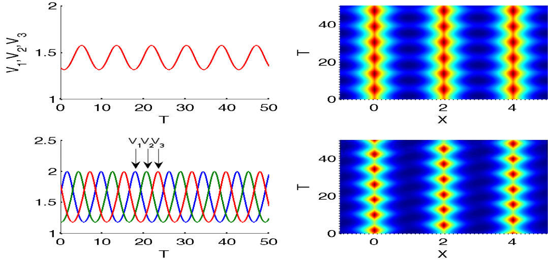
Figure 14: Full numerical results computed from (5.1) with D = 0.5 (upper row) and D = 0.2 (lower row). Other parameters are the same as in Fig. 12 with \kappa = 1 . The initial conditions for D = 0.5 are V_0 = [0.5, 1.5, 0.5] , W_0 = [1, 1, 1] , and C_0(x) = 1 . For D = 0.2 the initial conditions are V_0 = [0.5, 1.5, 0.5] , W_0 = [1, 1, 1] , and C_0(x) = 1 if x > 0 , C_0(x) = \sin(x) + 1 if x < 0 . The V_1 , V_2 and V_3 curves are labeled in the lower left figure. For D = 0.5 there are stable in-phase synchronous oscillations, whereas for D = 0.2 stable splayphase synchronous oscillations occur. The phase shift among V_1 , V_2 and V_3 , is consistent with the mode l = 2 in (5.14). The right panel in each row is a contour plot of C(x, t) .
