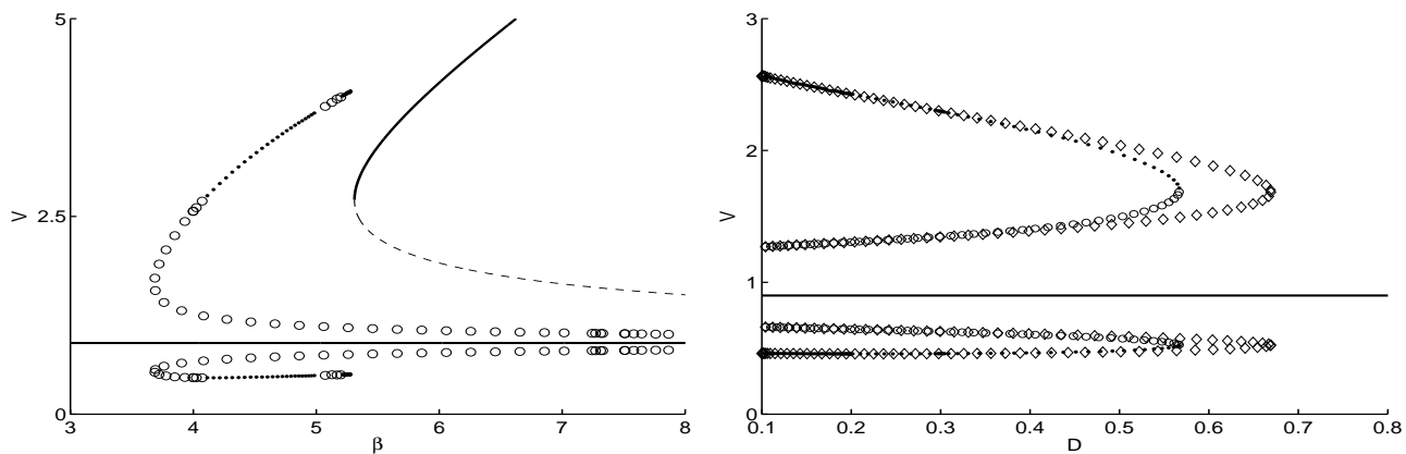
Figure 8: Bifurcation diagram of the local variable V with respect to the coupling strength \beta and diffusivity D for the parameter set L = 1 , k = 2 , \kappa = 3 , \epsilon = 0.15 , \mu = 0.9 , \alpha = 0.55 , K_c = 1 and L_v = 0.8 . The solid/dashed line represents stable/unstable steady-state solutions of V , open/solid circles indicate unstable/stable periodic solutions branches, respectively. The steady-state (4.5) is the solid horizontal line. Left panel: V versus \beta for D = 0.1 . The periodic solution branches shown correspond only to the in-phase oscillations. Stable in-phase synchronous oscillations and stable steady-states will co-exist only for some range of \beta . Right panel: V versus D for \beta = 4 . The periodic solution branch that is unstable, with a saddle-node point at D \approx 0.67 , is the in-phase branch. The other periodic solution branch, with a saddle-node point at D \approx 0.57 represents anti-phase oscillations. This plot shows that in-phase oscillations are unstable for \beta = 4 , but that stable anti-phase oscillations and stable steady-state solutions will co-exist in some range of D when \beta = 4 .
