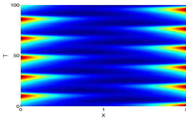
Figure 9: Numerical simulation of the coupled PDE-ODE system (2.1) with the nonlinear coupling (4.1) for D = 0.5 , \beta = 4 , and L = 1 . The other parameter values are the same as in the caption of Fig. 8. The initial conditions are C(x, 0) = 2 , v_1 = 1 , w_1 = 0.3 , v_2 = 0.2 , and w_2 = 0.3 . Stable anti-phase oscillations for C(x, t) are observed.
