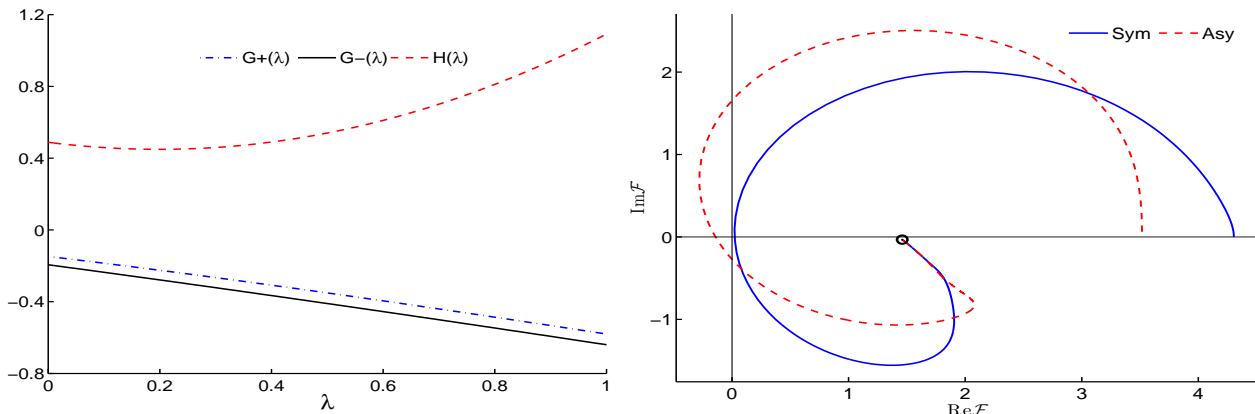
Figure 7: Left panel: G_+(\lambda) , G_-(\lambda) , and H(\lambda) , as defined in (3.7), plotted on \lambda > 0 real for D = 1 and \beta = 0.7 , with the other parameters as in the caption of Fig. 1. Since there is no intersection of G_{\pm}(\lambda) and H(\lambda) , then \mathcal{F}(\lambda) has no real roots \lambda for either the in-phase and anti-phase modes. Right panel: \mathcal{F}_I(\lambda_I) = \text{Im}(\mathcal{F}(i\lambda_I)) is plotted versus \mathcal{F}_R(\lambda_I) = \text{Re}(\mathcal{F}(i\lambda_I)) for both the in-phase and anti-phase modes as \lambda_I is decreased from 1000 to 0. The open circle is the starting point at \lambda_I = 1000 . For the anti-phase mode (dashed curve), we have m = -1 in (3.6) since the trajectory wraps around the origin once in the clockwise direction. For the in-phase mode (solid curve), the plot shows that m = 0 in (3.6).
