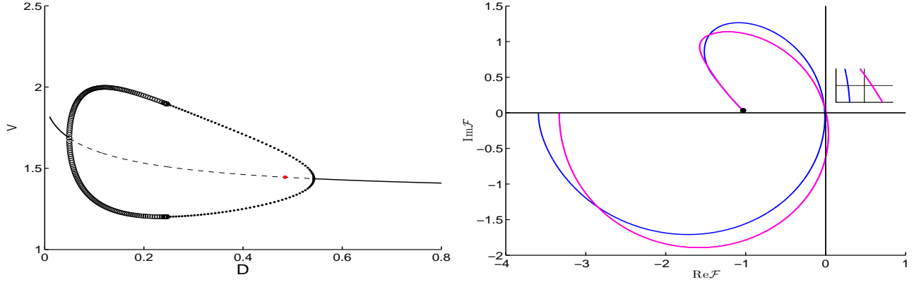
Figure 13: Left: Global bifurcation diagram with m = 3 cells on the domain [-1, 5] for \kappa = 1 , with the other parameters as in the caption of Fig. 12. The solid and dashed lines denote linearly stable and unstable branches of steady-state solutions, respectively. The closed loop is the global branch of in-phase periodic solutions. The upper Hopf bifurcation value D \approx 0.54299 is for the l = 0 in-phase mode. The solid/open circles on this loop denote a linearly stable/unstable periodic solution, respectively. The dot at D \approx 0.48482 is the Hopf bifurcation point for the degenerate l = 1, 2 mode. Right panel: Plot of \mathcal{F}(i\lambda_l) as \lambda_l decreases from 1000 to 0 with D = 0.5 . The curve that crosses slightly into the region \text{Re}\mathcal{F} > 0 (see the inset for curves near the origin) is the l = 1, 2 mode, while the other curve is for l = 0 . The trace and determinant of J_e are \text{tr}J_e = 0.4879 and \det J_e = 0.4474 , so that P = 2 in (5.15). We obtain N = 2 unstable eigenvalues for l = 0 , and N = 0 for l = 1, 2 from (5.15).
