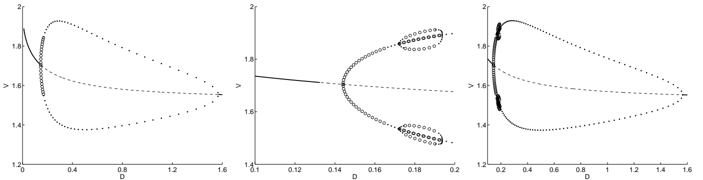
Figure 3: Bifurcation diagram of V versus D when \beta = 0.6325 (left) and \beta = 0.635 (middle), corresponding to taking a vertical slice in the phase diagram of Fig. 1. The loops in these figures are for in-phase periodic solutions only, with open/closed circles denoting unstable/stable solutions. These \beta values are slightly to the right of the end of the faint-dashed curve in Fig. 1. The plot on the right for \beta = 0.635 is the same as for the middle plot except it is for a larger range of D . For \beta = 0.6325 we observe that the in-phase branch is stable except near the Hopf bifurcation point on the steady-state branch. However, for \beta = 0.635 the in-phase periodic solution branch has a much more intricate bifurcation structure.
