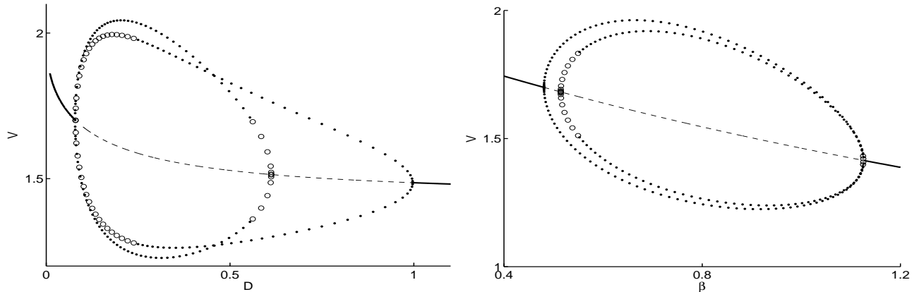
Figure 2: Bifurcation diagram of V corresponding to the vertical and horizontal slices through the phase diagram of Fig. 1, as computed using XPPAUT [7]. Left panel: V versus D for \beta = 0.8 (vertical slice). Right panel: V versus \beta for D = 0.4 (horizontal slice). The solid and dashed lines denote linearly stable and unstable branches of steady-state solutions, respectively. The two closed loops correspond to branches of in-phase and anti-phase periodic solutions. In the left panel, the branch that bifurcates from the steady-state near D = 1 is the in-phase synchronous branch and in the right panel, the outer loop is the anti-phase branch. The solid/open circles on these loops denote linearly stable/unstable periodic solutions, respectively. The other parameters are as in the caption of Fig. 1.
