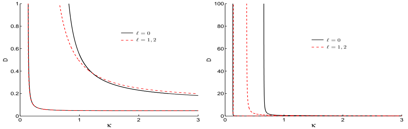
Figure 12: Left: Phase diagram showing Hopf bifurcation boundaries for the case of three ( m = 3 ) cells in the D versus \kappa plane for k = 1 , L = 1 , and where the Sel'kov parameters in (2.1c) are \epsilon = 0.15 , \mu = 2 and \alpha = 0.9 . The solid curves corresponds to l = 0 and the dotted curves corresponds to l = 1, 2 . The two curves almost coincide on the lower boundary. In the region bounded by the two solid and two dotted curves the symmetric steady-state is linearly unstable to the l = 0 and l = 1, 2 modes, respectively. Right: Same as the left panel, but with a larger range of D for the vertical axis. For these parameter values we observe that the region of instability is unbounded in the D versus \kappa plane.
