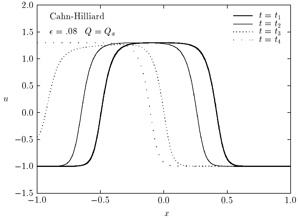
Figure 3: Plots of the numerical solution to the Cahn-Hilliard equation at different times corresponding to the parameter values given in the caption of Table 1b. The times are t_1 = 22.4 , t_2 = 1.3912861374 \times 10^{11} , t_3 = 1.3913503805 \times 10^{11} , and t_4 = 1.3921798980 \times 10^{11} . The internal layer centered at x = x_0 collapses when t \approx t_3 . The duration of this collapse process is presumably O(1) .
