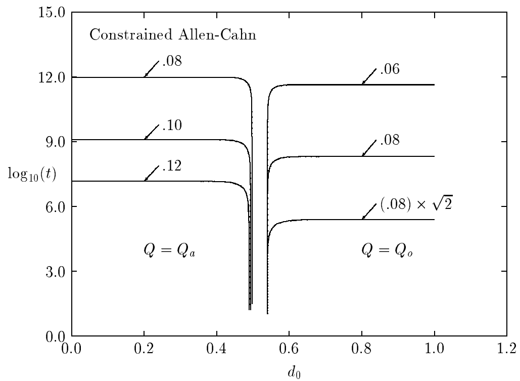
Figure 4: Same caption as for figure 2 except that plots of \log_{10}(t) versus d_0 are now shown for the constrained Allen-Cahn equation ( \alpha = 1 and \kappa = 1 ).
