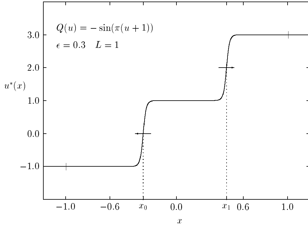
Figure 6: Plot of u^*(x) given by (5.2) with u_s(z) = 4\pi^{-1} \tan^{-1}(e^{z\pi^{1/2}}) - 1 and s = 1 that approximates a two-layer metastable pattern for (5.1). The artificial boundary conditions (5.1b) are applied at L = 1 . On the infinite line, the motion of the internal layers for all time is in the direction of the arrows.
