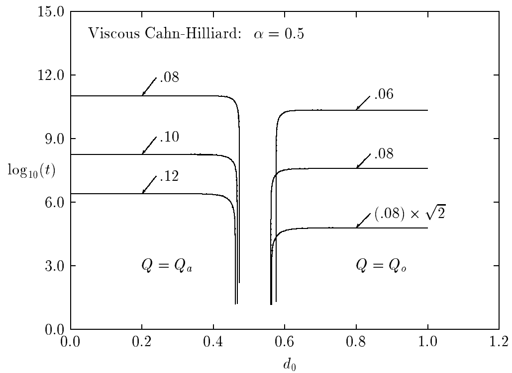
Figure 5: Same caption as for figure 2 except that plots of \log_{10}(t) versus d_0 are now shown for the viscous Cahn-Hilliard equation with \alpha = 0.5 and \kappa = 1 .
