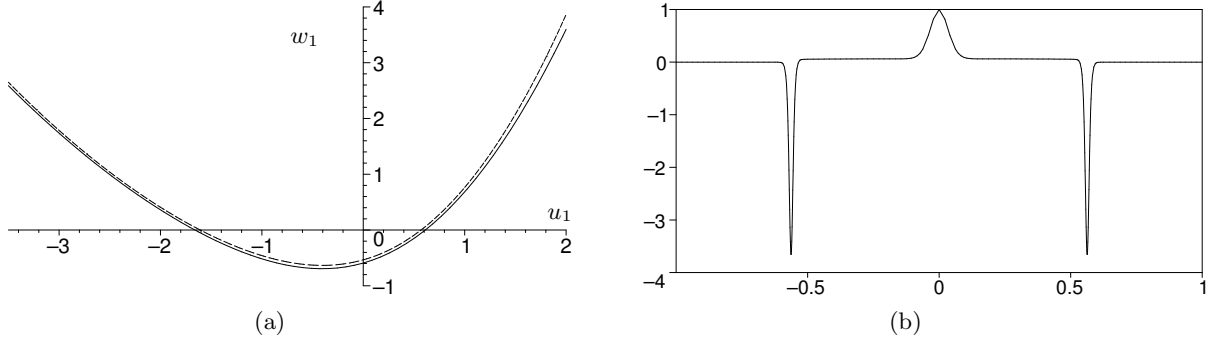
FIGURE 6. (a) The plot of u_1 versus w_1(0) computed from (3.5). The solid and dashed lines correspond to numerical computations of the full steady-state system (2.3) and the core problem (3.4), respectively. (b) The dimple eigenfunction \phi at the fold point. The parameter values are \varepsilon = 0.005 , \beta_0 = 1.5 , with D determined numerically as a function of u_1(0)
