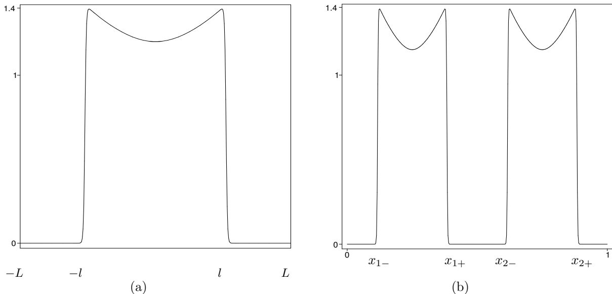
FIGURE 2. (a) A single mesa steady-state on [-L, L] . The parameter values are L = 1 , \beta_0 = 1.5 , D = 1.29 , \varepsilon = 0.005 . (b) A two-mesa steady state ( K = 2 , L = 1/4 , x \in [0, 1] ). The parameter values are D = 0.068 , \varepsilon = 0.00125 , \beta_0 = 1.5 .
